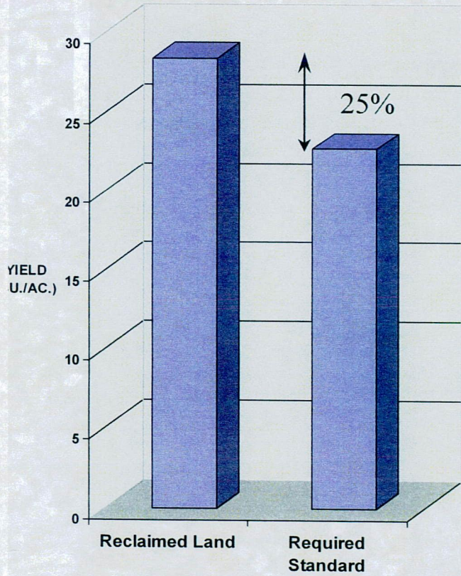
CROPLAND PRODUCTIVITY
