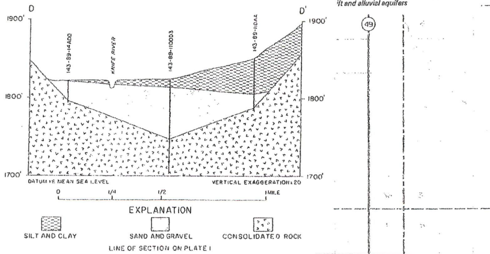
FIGURE 22.--Geologic section D-D' through the Knife River aquifer, Mercer County.
