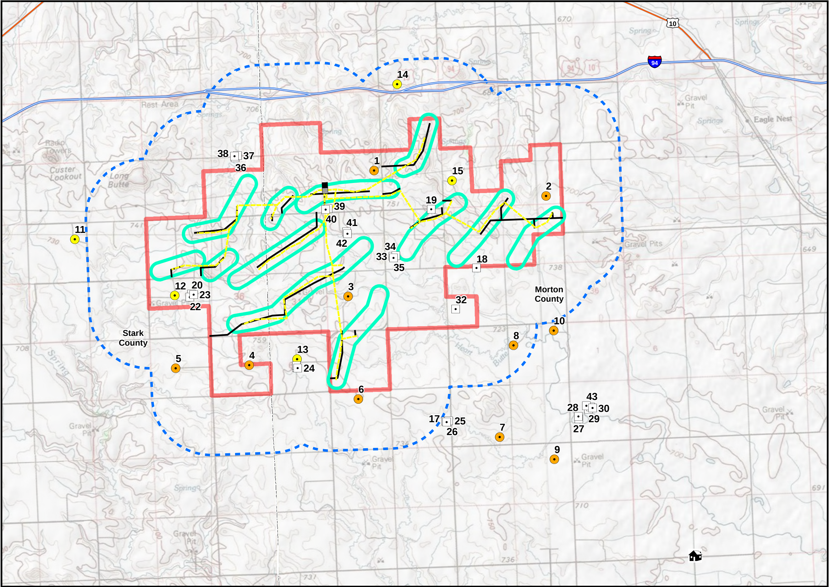
Figure 10 Noise and Shadow Flicker Sensitive Receptors
