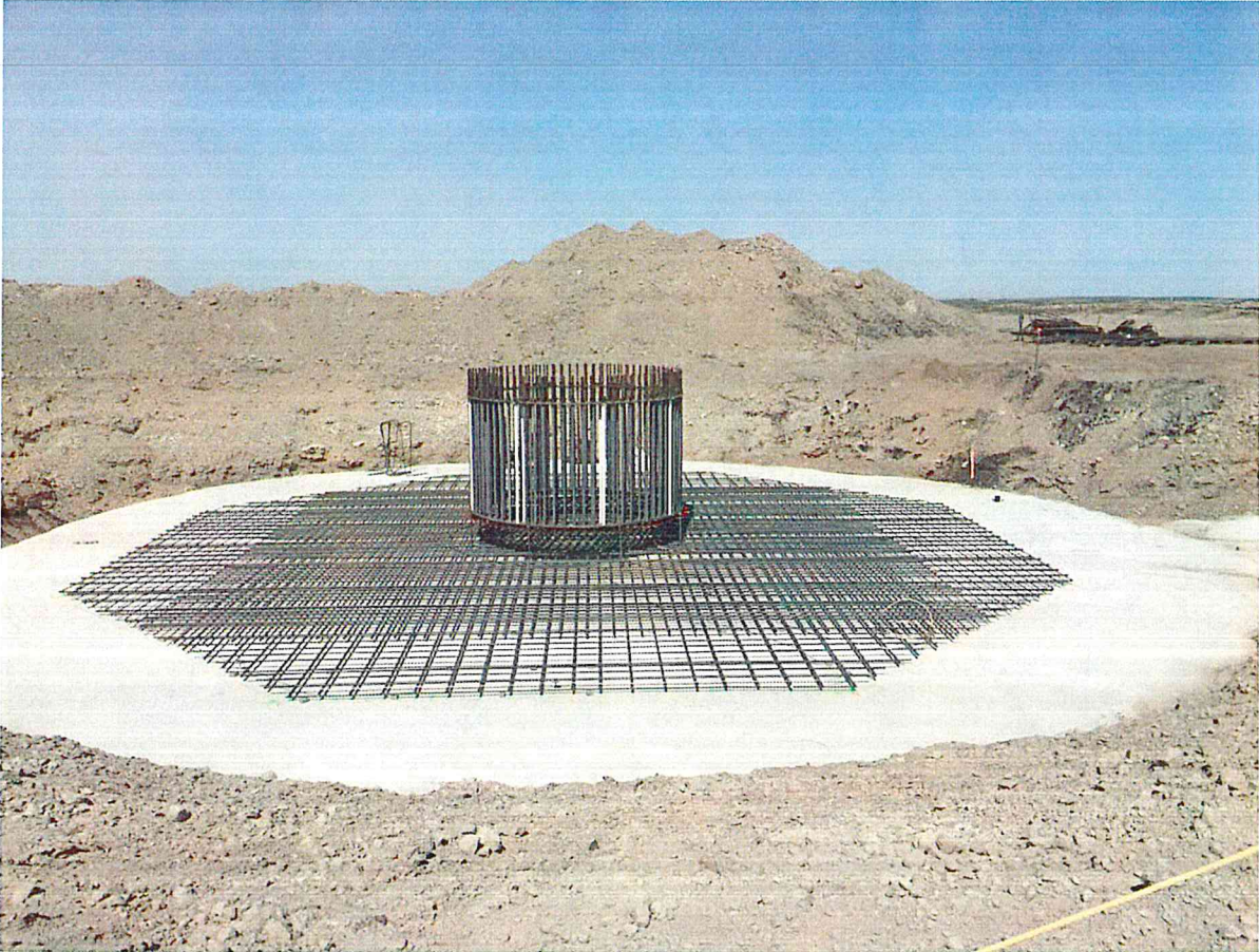
Bottom Mat and Anchor Bolt Cage
