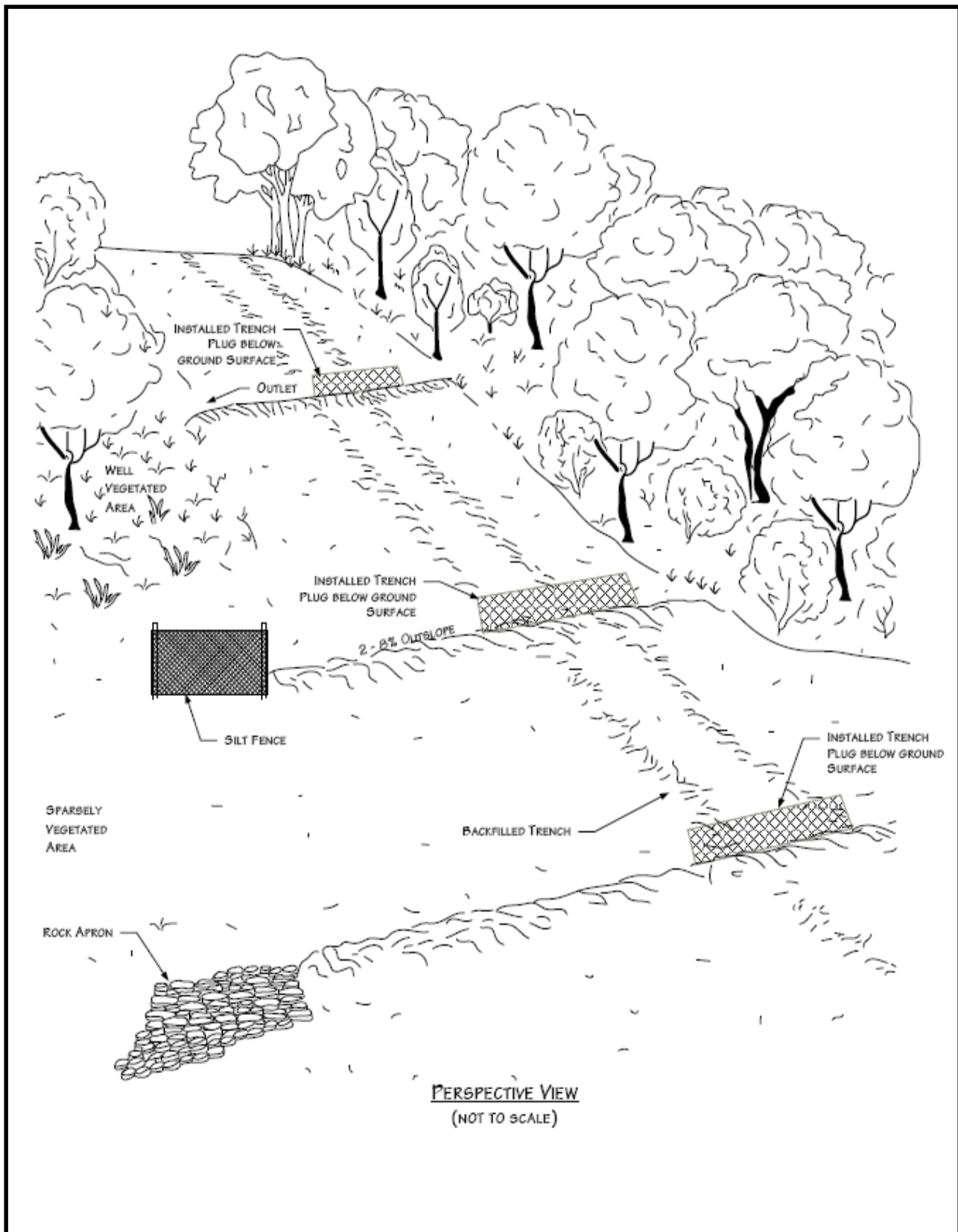
Figure 6.7.1 – Permanent Slope Breakers Perspective View
