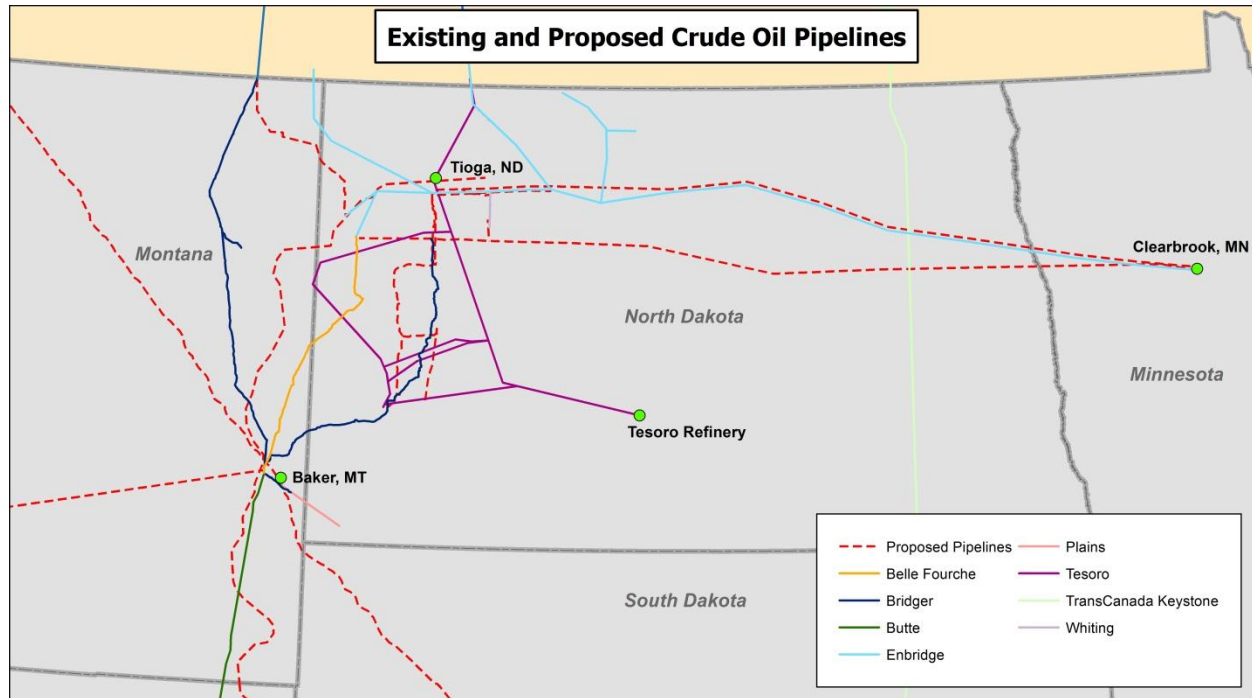
Figure 27: Existing and Proposed Crude Oil Pipelines
