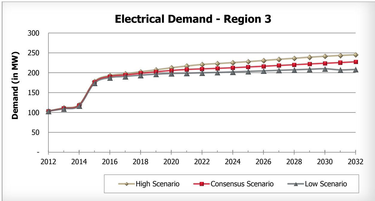
Figure 9: Electrical Demand - Region 3
