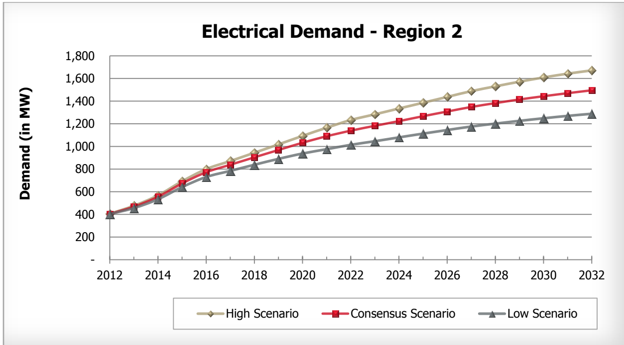
Figure 8: Electrical Demand - Region 2
