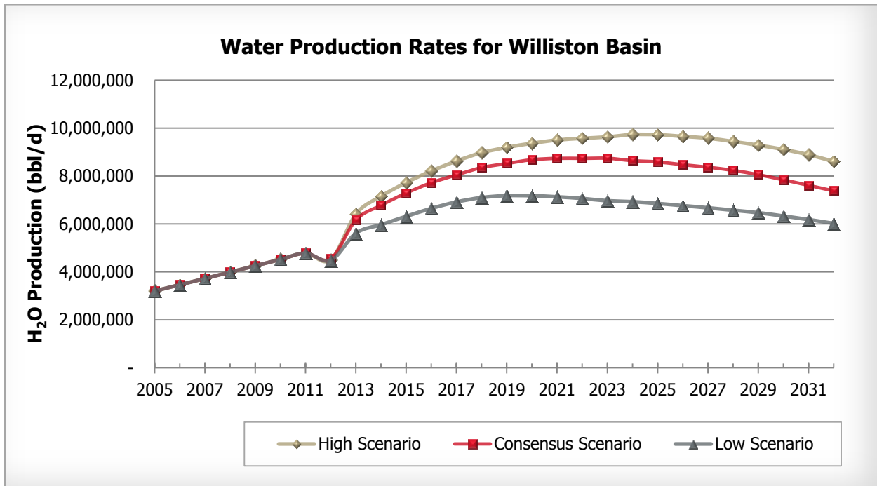
Figure 19: Water Production Rates for Williston Basin
