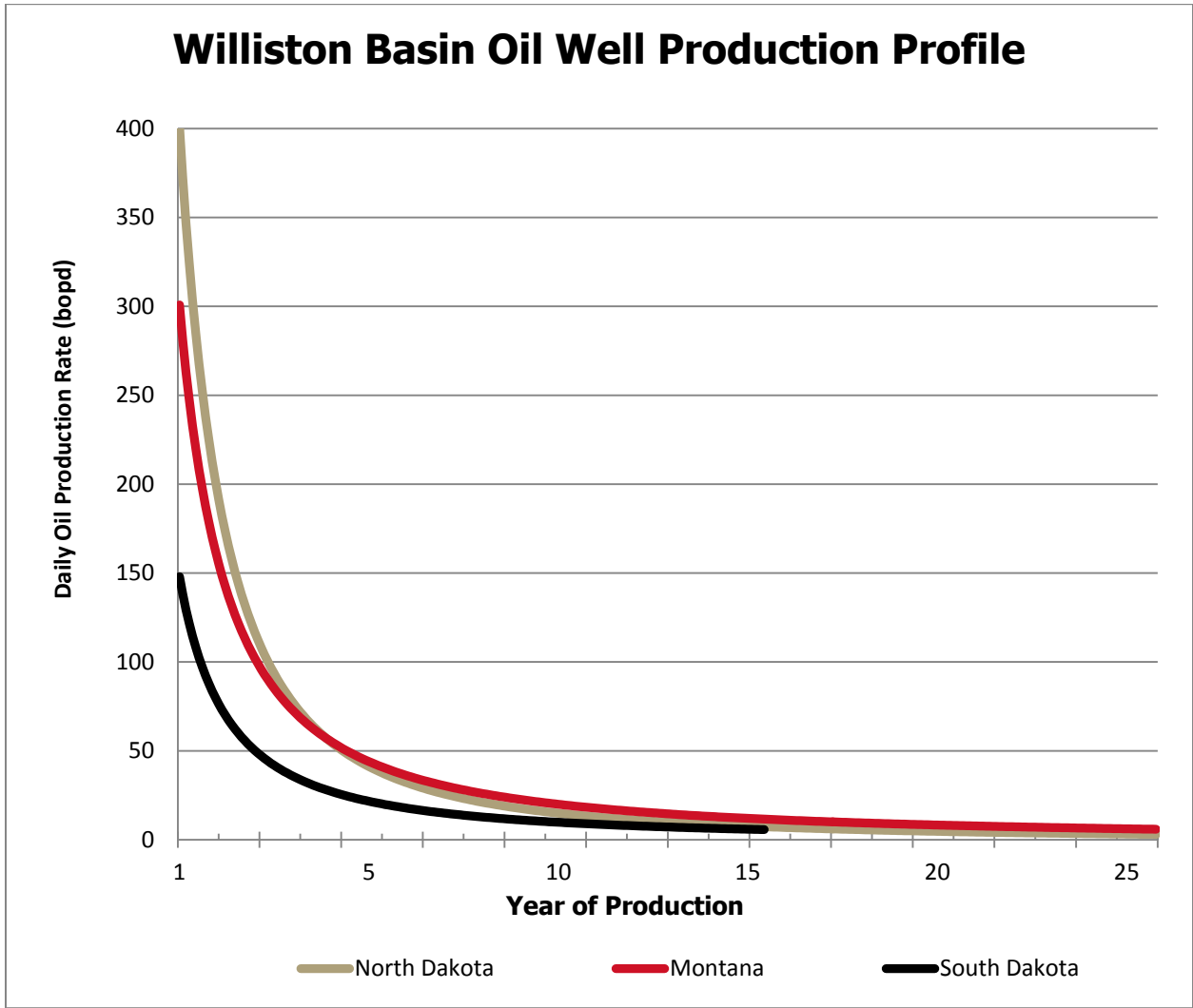
Figure 25: Williston Basin Oil Well Production Profiles Source: University of North Dakota
