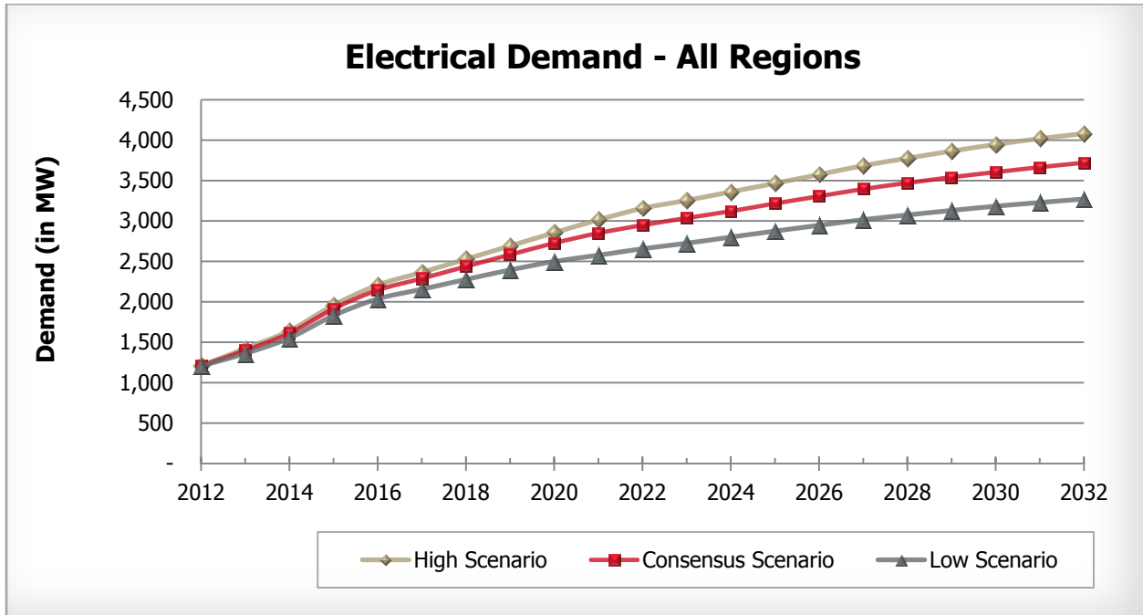
Figure 10: Electrical Demand - All Regions
