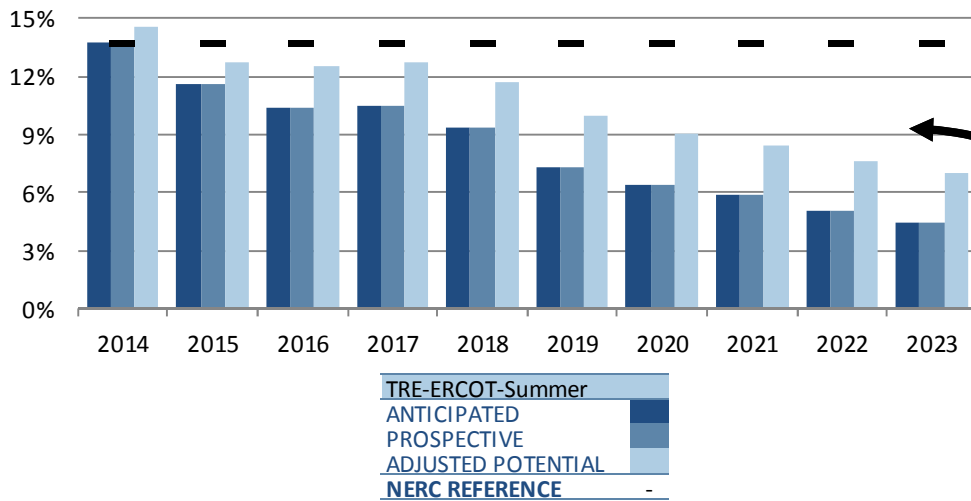
ERCOT Planning Reserve Margins
