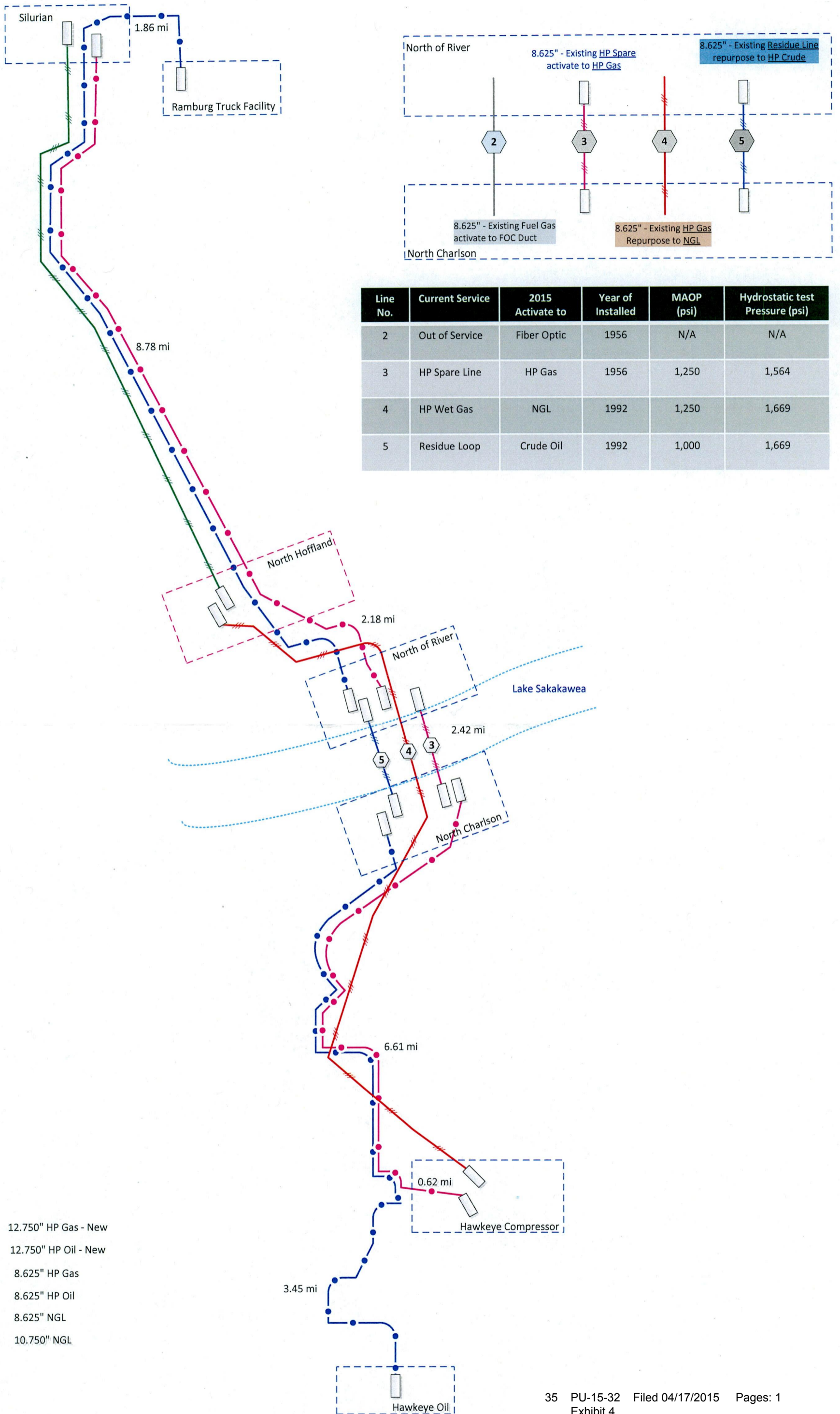
Figure 2 Schematic Depiction of the Proposed Hawkeye Pipeline System Project
