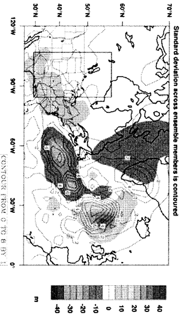
b Ensemble average geopotential height anomaly at 510mb (4.5 days)
