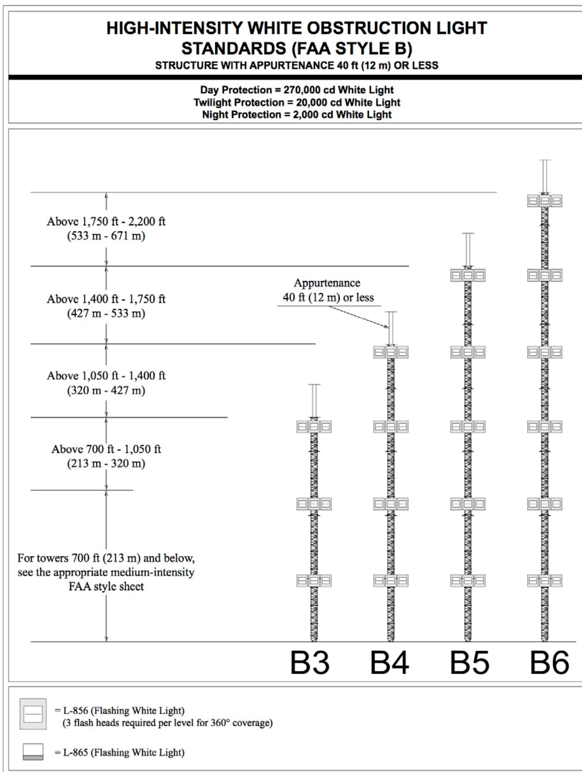
Figure A-8. High-Intensity White Obstruction Light Standards—Structures With Appurtenance 40 Feet or Less
