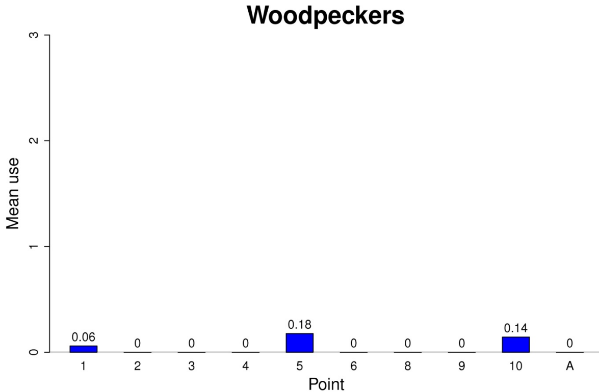
Figure 2 (continued). Mean use (number of birds/20-min survey) at each fixed-point bird use survey point for all birds and major bird types at the Glacier Ridge Wind Project. Observations of passerines and other small birds were focused within 100-m viewsheds.
