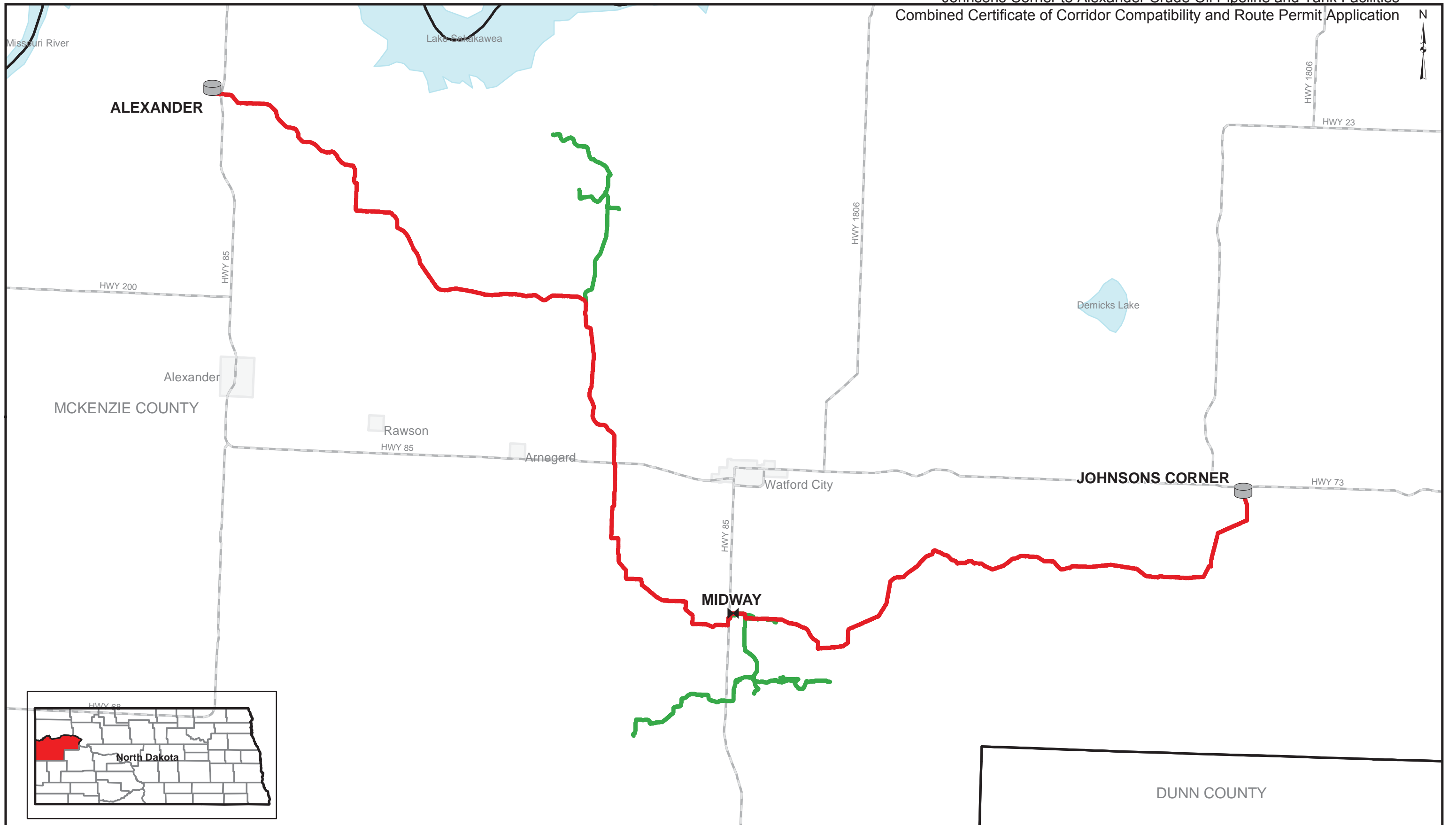
Figure 5 Targa Pipeline System
