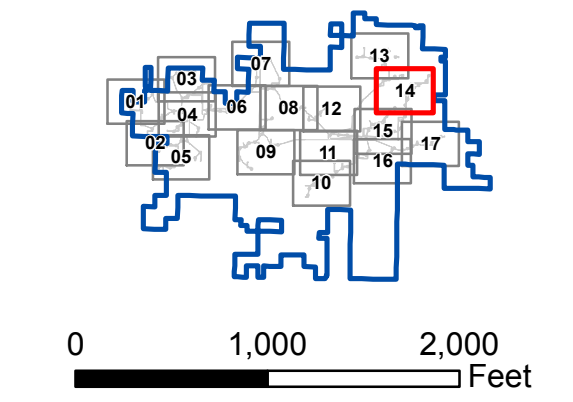
Infrastructure and Occupied Residences Map 14 of 17 Emmons-Logan Wind Energy Center Emmons and Logan Counties, ND
