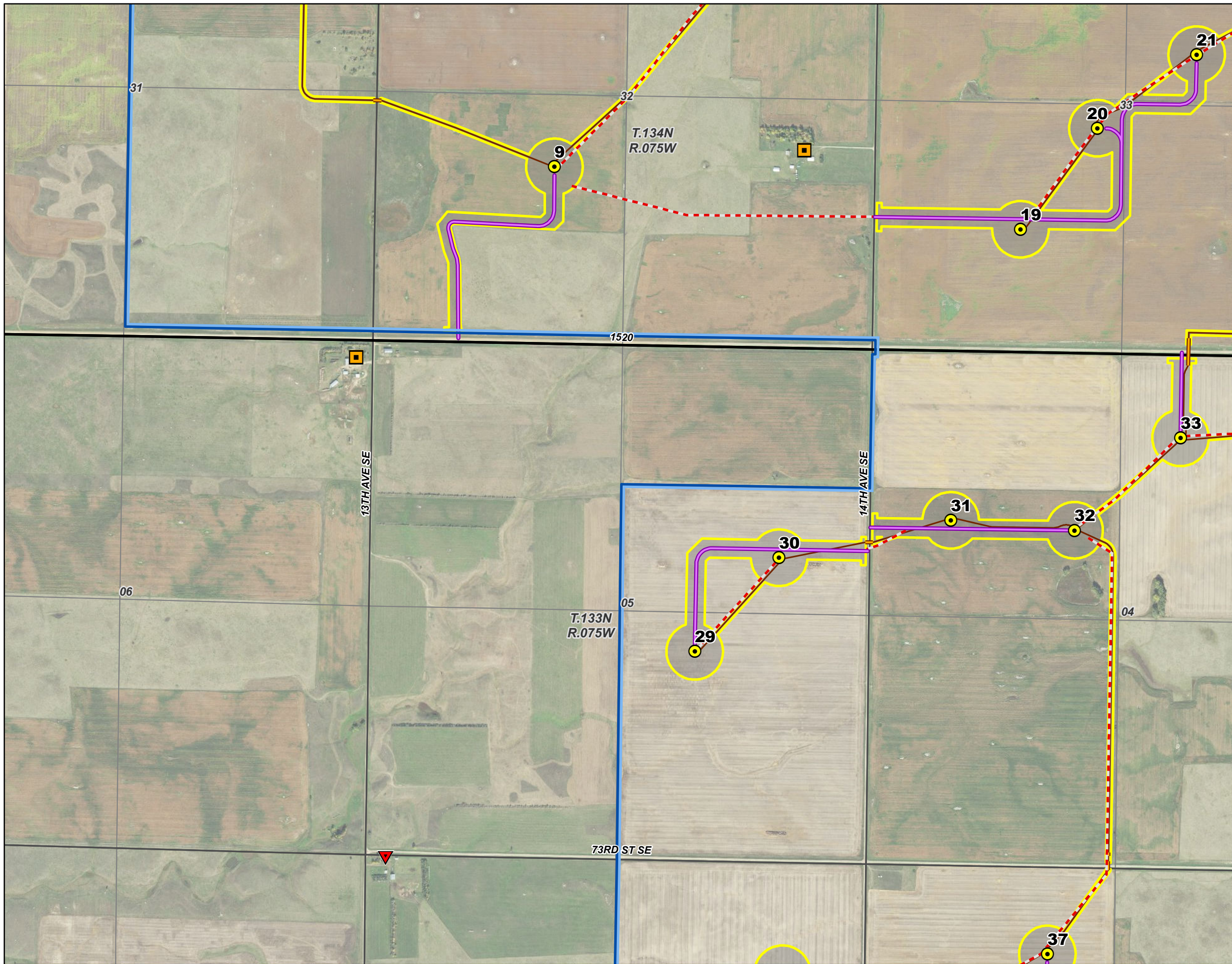
Infrastructure and Occupied Residences Map 2 of 17 Emmons-Logan Wind Energy Center Emmons and Logan Counties, ND
