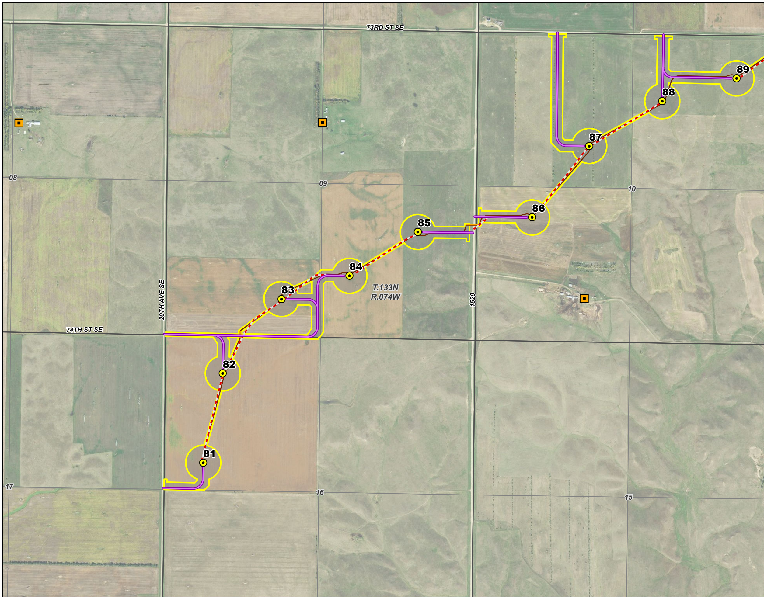
Infrastructure and Occupied Residences Map 10 of 17 Emmons-Logan Wind Energy Center Emmons and Logan Counties, ND
