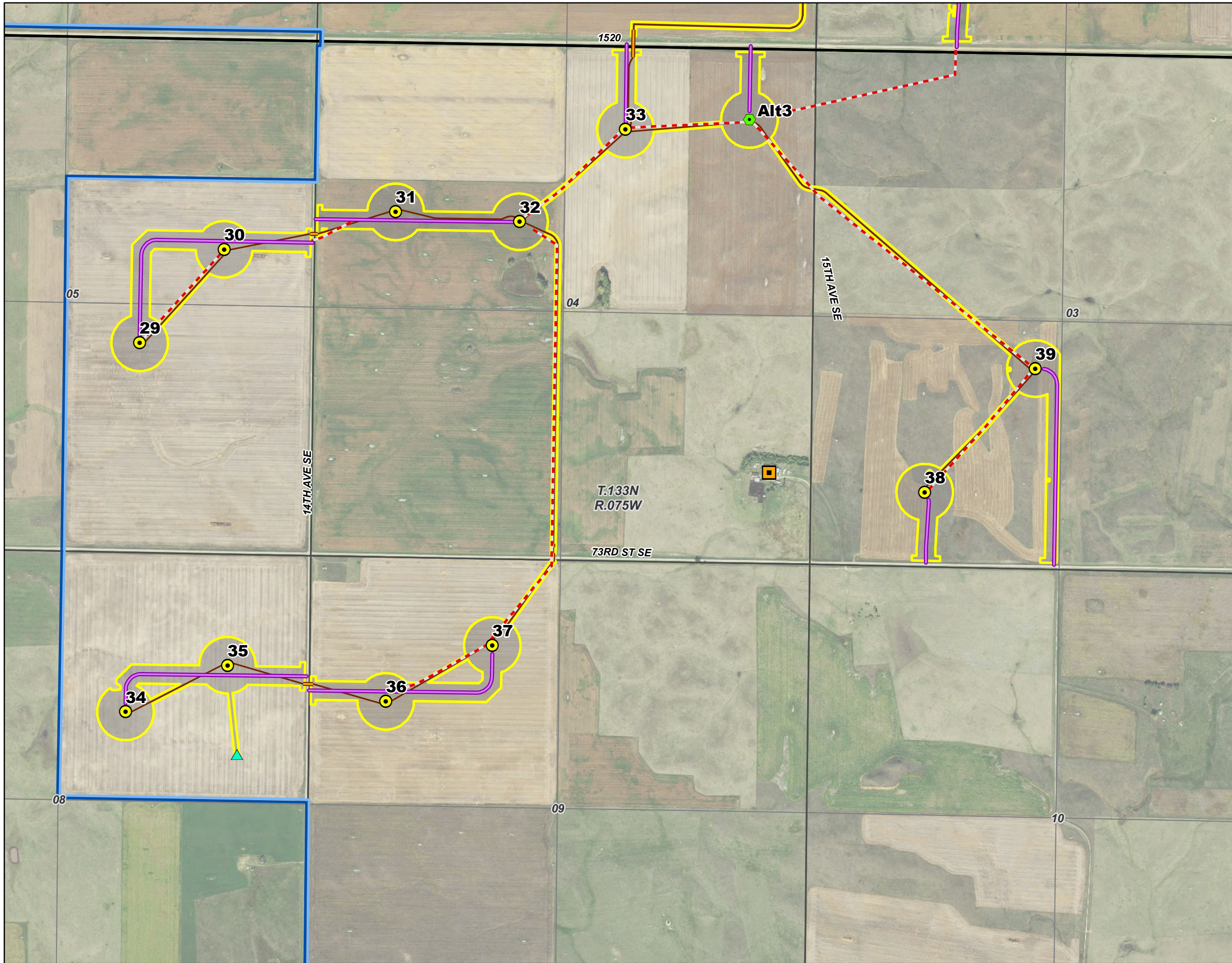
Infrastructure and Occupied Residences Map 5 of 17 Emmons-Logan Wind Energy Center Emmons and Logan Counties, ND
