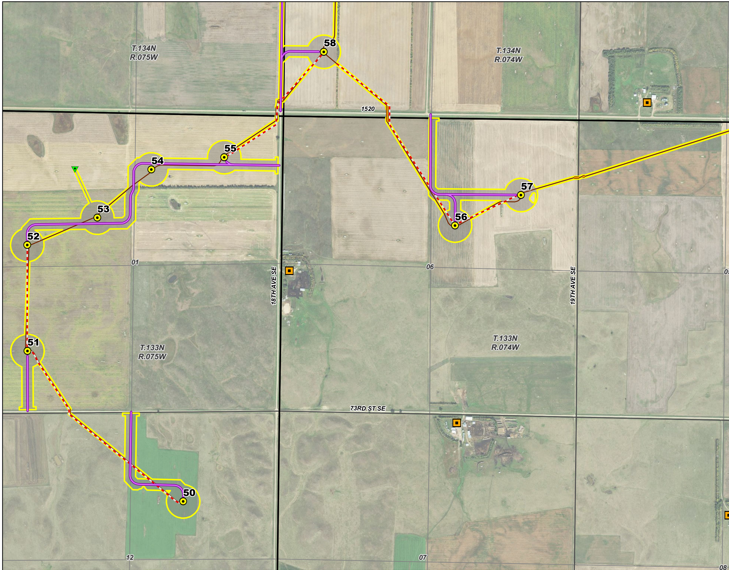
Infrastructure and Occupied Residences Map 9 of 17 Emmons-Logan Wind Energy Center Emmons and Logan Counties, ND
