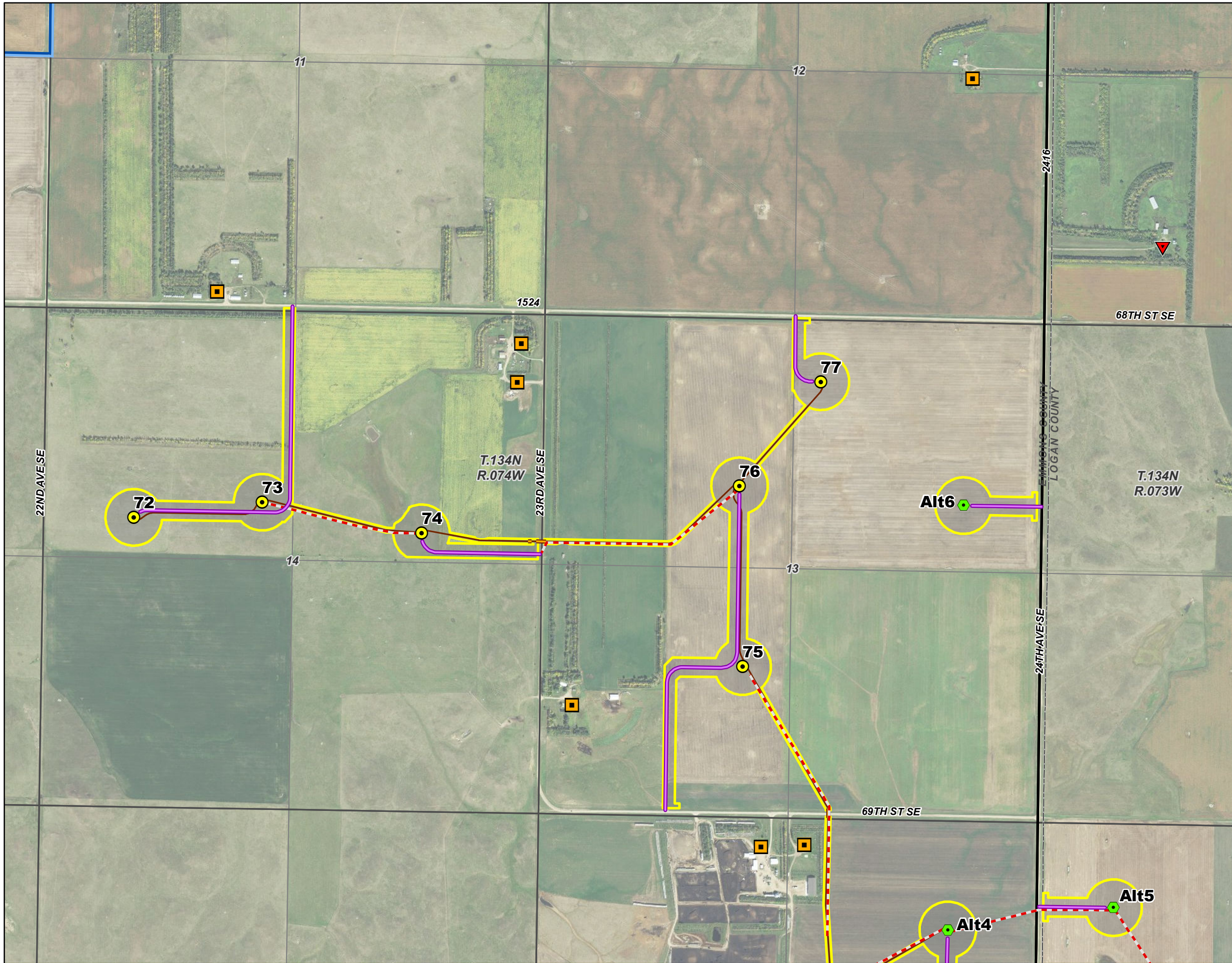
Infrastructure and Occupied Residences Map 13 of 17 Emmons-Logan Wind Energy Center Emmons and Logan Counties, ND
