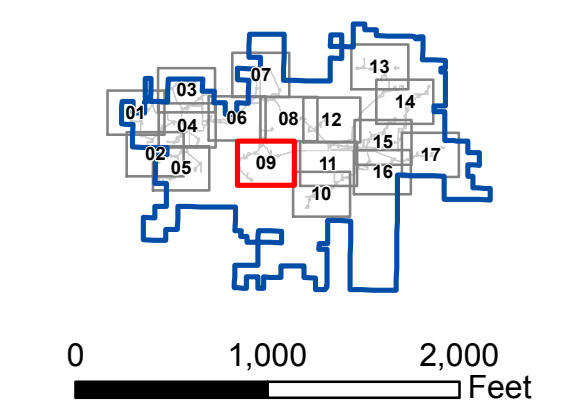
Infrastructure and Occupied Residences Map 9 of 17 Emmons-Logan Wind Energy Center Emmons and Logan Counties, ND
