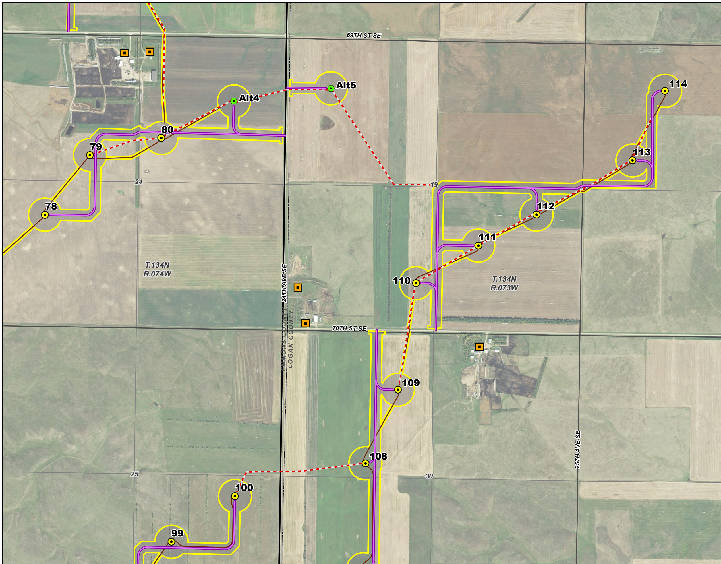
Infrastructure and Occupied Residences Map 14 of 17 Emmons-Logan Wind Energy Center Emmons and Logan Counties, ND
