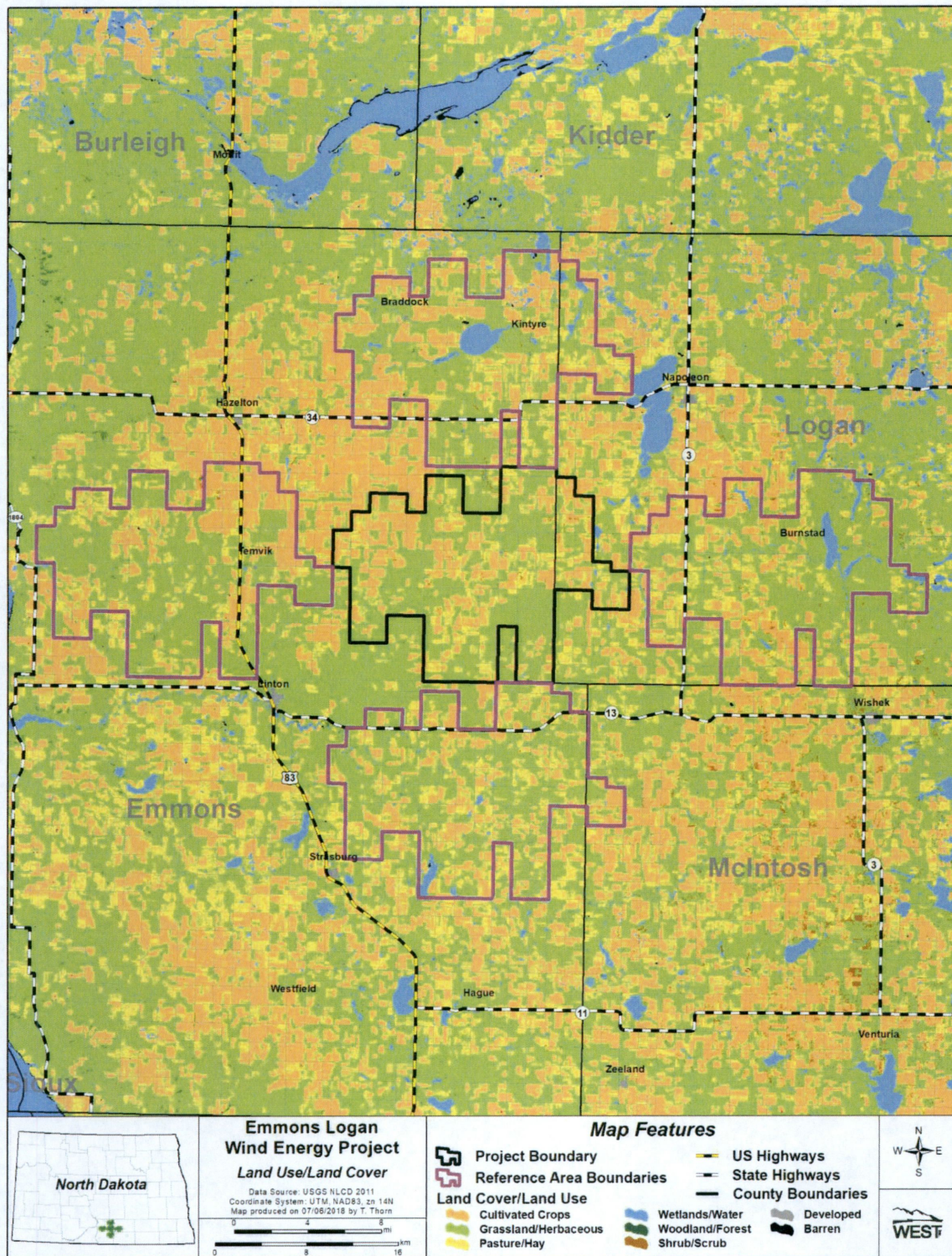
Figure 2. Land Use/Land Cover within and around the Emmons-Logan Wind Project and adjacent reference areas.
