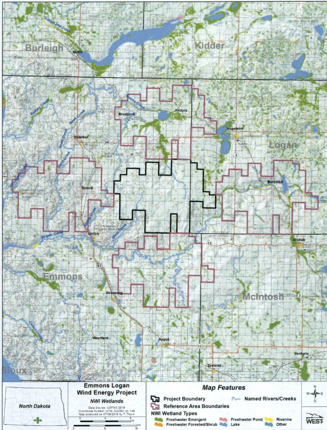
Figure 3. NWI wetlands and rivers/creeks within and around the Emmons-Logan Wind Project and adjacent reference areas.
