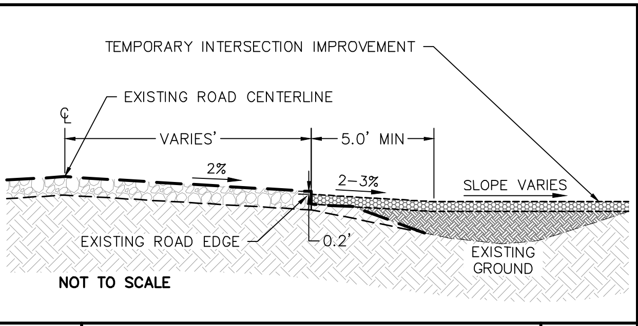
Westwood TEMPORARY INTERSECTION IMPROVEMENT TYPICAL SECTION RD30
