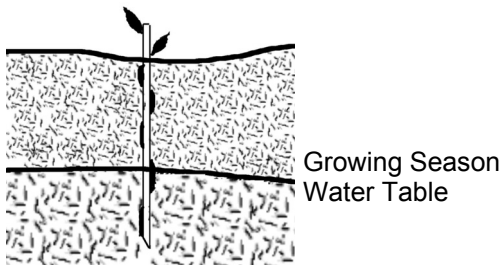
Figure 7: Unrooted Cutting
