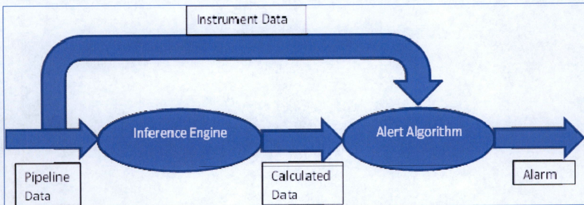
Figure 7.1 Typical CPM System per API 1130
