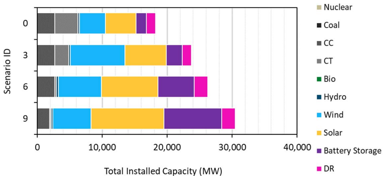
Figure 5-11. 2045 snapshot: installed capacity (MW) for Scenarios 3, 6 & 9
