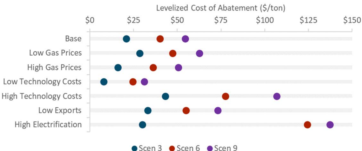
Figure 5-15. Sensitivity analysis on levelized cost of abatement across scenarios
