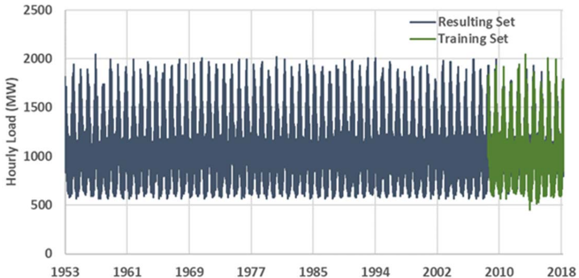
Figure A-3. Example of results of neural network regression to extend load across long weather record
