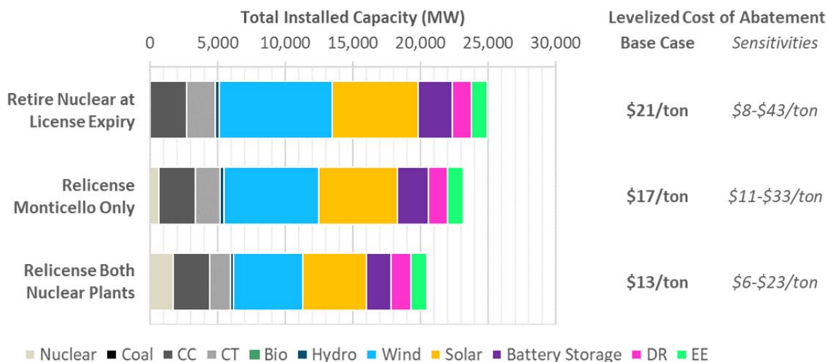
Figure vi. Xcel resource portfolios that achieve 95% carbon reductions in 2045
