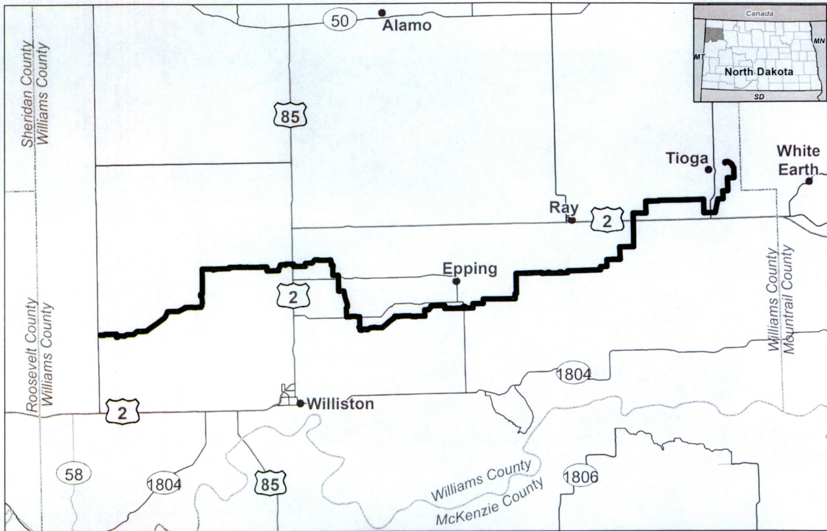
Exhibit B.5 ONEOK Bakken Pipeline, L.L.C. Tioga Lateral Pipeline Project Project Location Map
