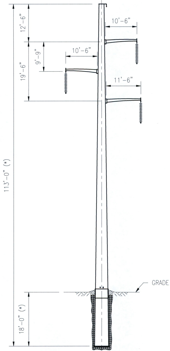
BASIC 230KV SINGLE CIRCUIT STRUCTURE (*) LENGTH VARIES - SEE PLAN AND PROFILE
