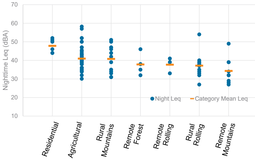
FIGURE 5: BACKGROUND NIGHTTIME L_{eq} AT 102 LOCATIONS AT POTENTIAL WIND TURBINE SITES ACROSS THE U.S. BY LAND USE CATEGORY 3
