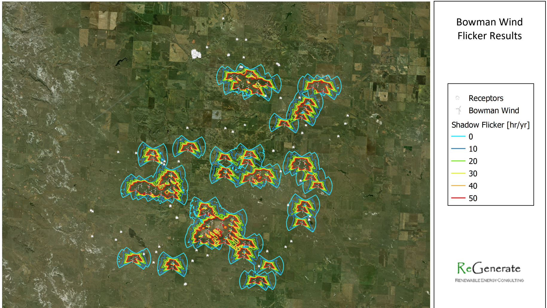
Figure 3: Shadow Flicker Map of Bowman Wind Project
