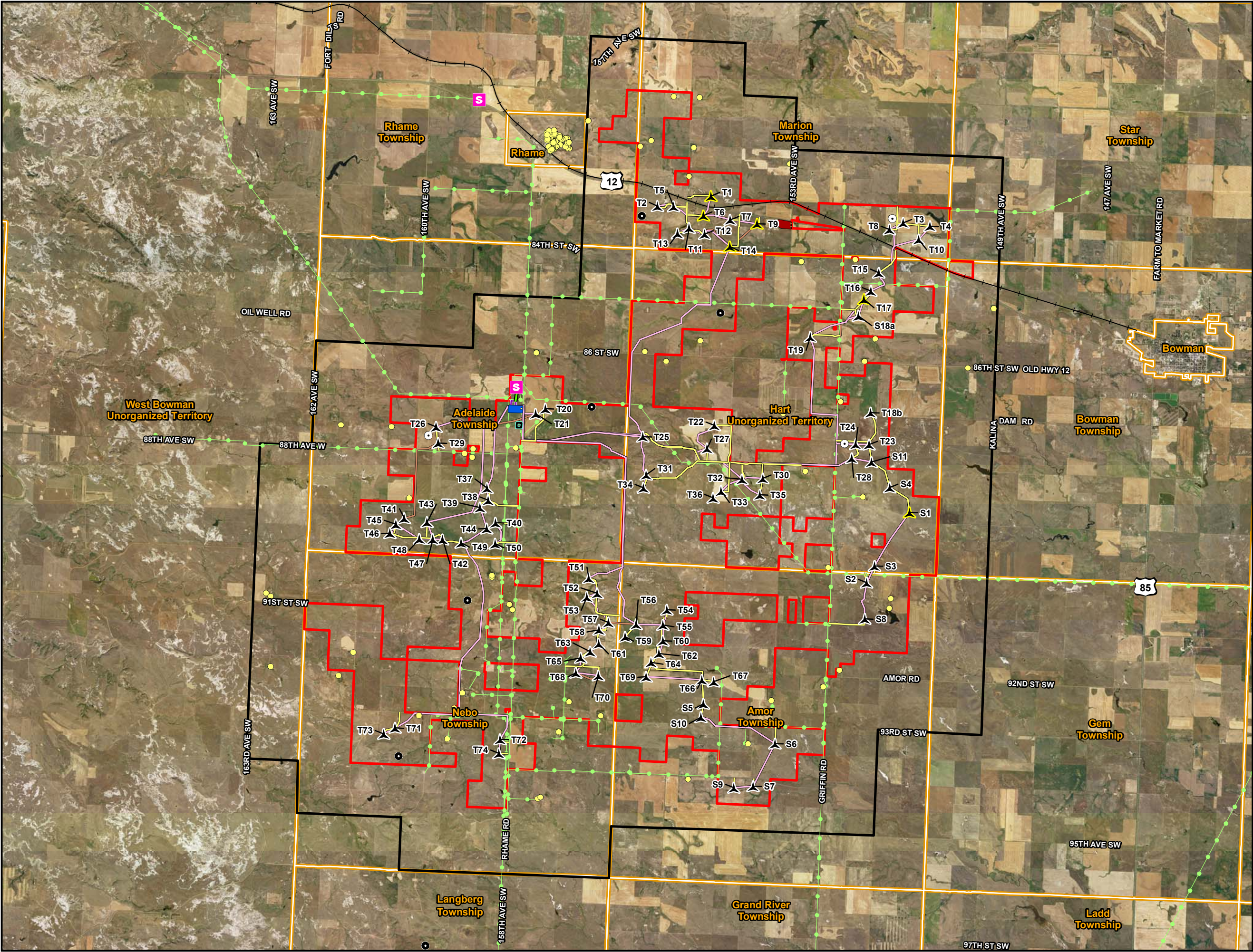
Figure 1 Facilities Layout Bowman Wind Project Bowman County, North Dakota
