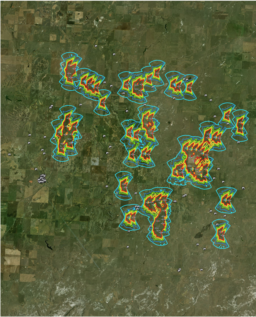
Figure 3: Shadow Flicker Map of Bowman Wind Project
