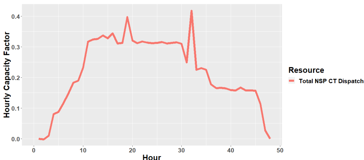
Figure 2-5: NSP System CT Dispatch Profile During Multi-Day Polar Vortex Event – January February 7-8, 2021
