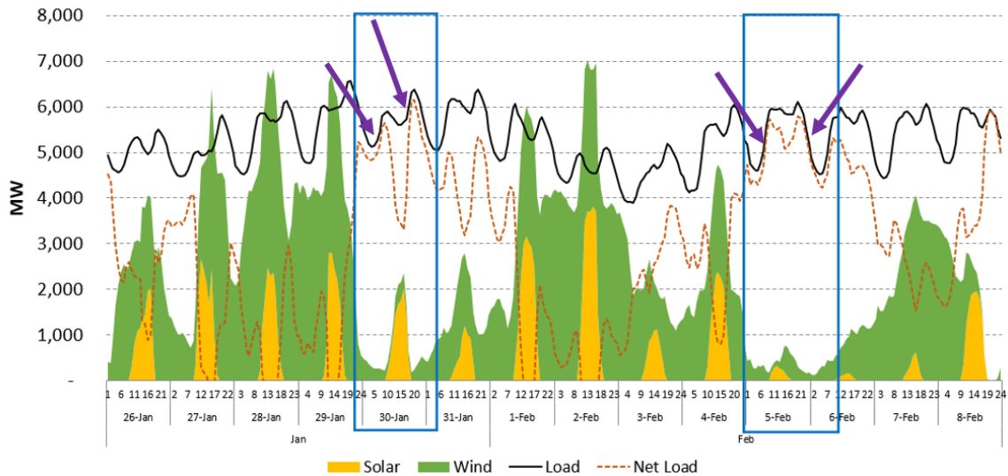
Figure 2-2: Approximated NSP System Output – 2019 Polar Vortex
