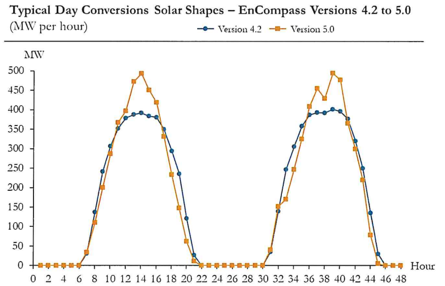
Figure 4-2: Typical Day Conversions for Solar Shapes, EnCompass Versions 4.2 versus 5.0
