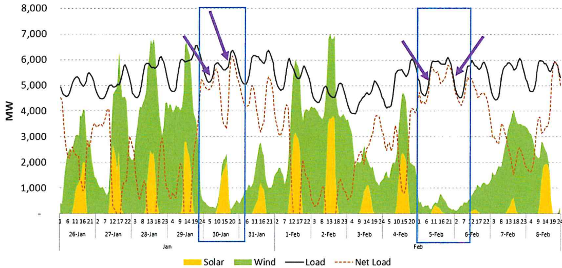
Figure 2-2: Approximated NSP System Output – 2019 Polar Vortex
