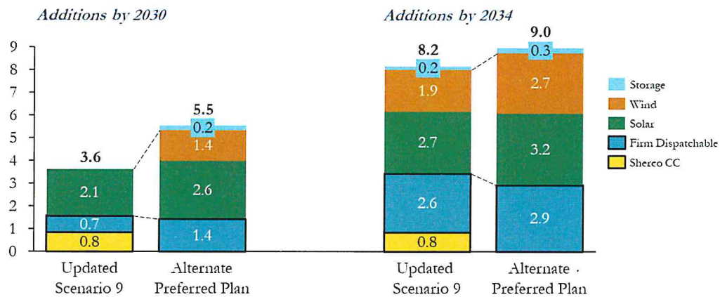
Large-Scale Capacity Additions in Updated Scenario 9 and Alternate Plan (GW of additions)
