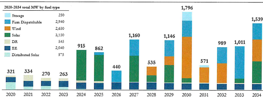
Alternate Plan Annual Expansion Plan (MW of additions)
