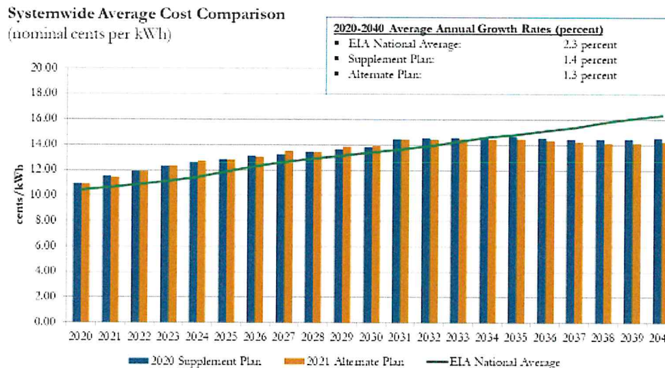
Figure 5-2: Systemwide Nominal Cost Comparison
