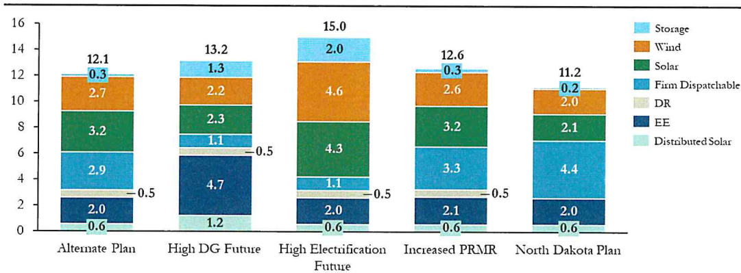
Alternate Plan Total Capacity Additions Under Special Case Assumptions, 2020-2034 (GW, UCAP)
