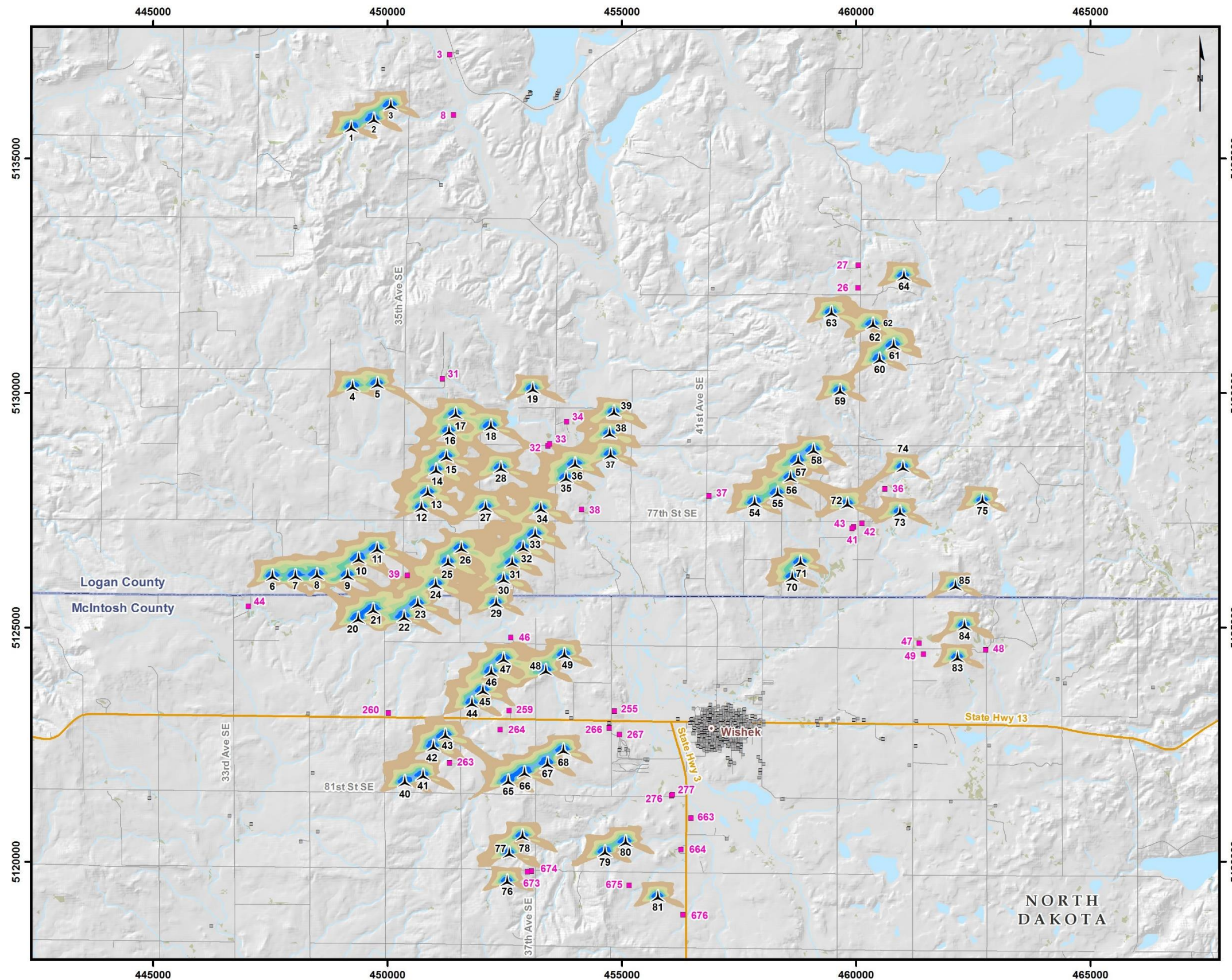
Figure 4-1 Modeled hours of shadow flicker (Expected Case)
