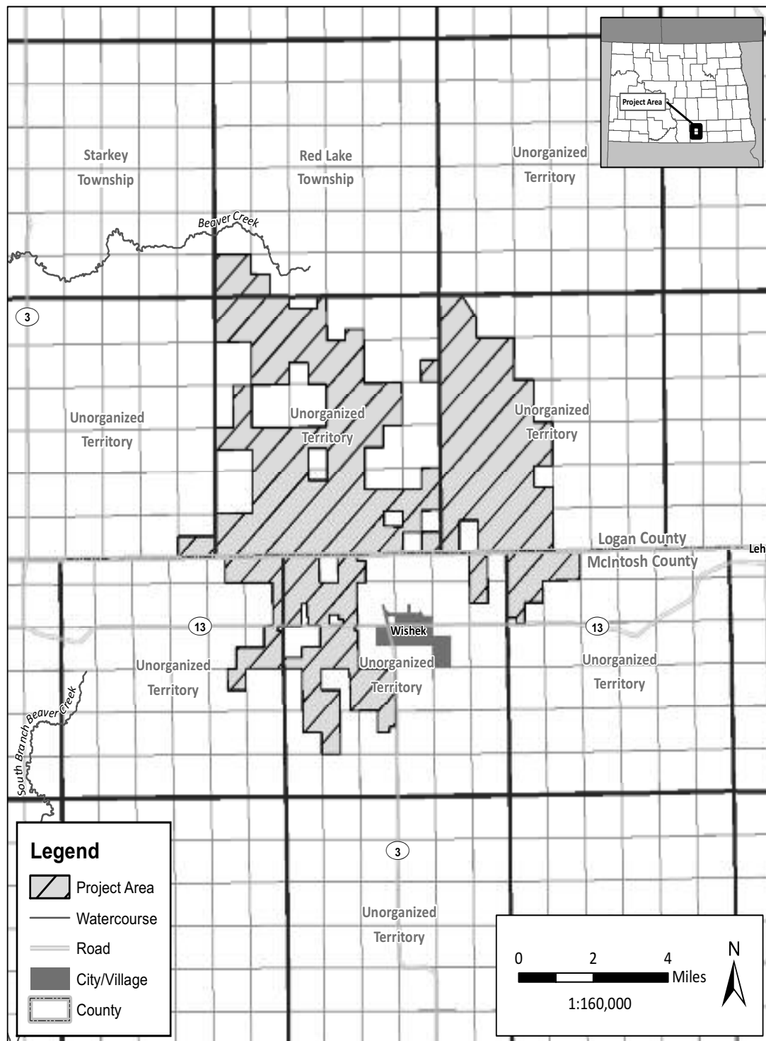
Figure 12 Badger Wind Project Logan and McIntosh Counties, North Dakota
