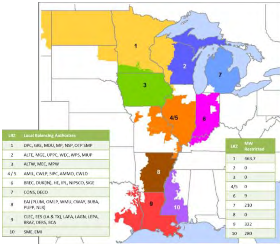
Figure 4.5-2: Local Resource Zones (LRZ)
