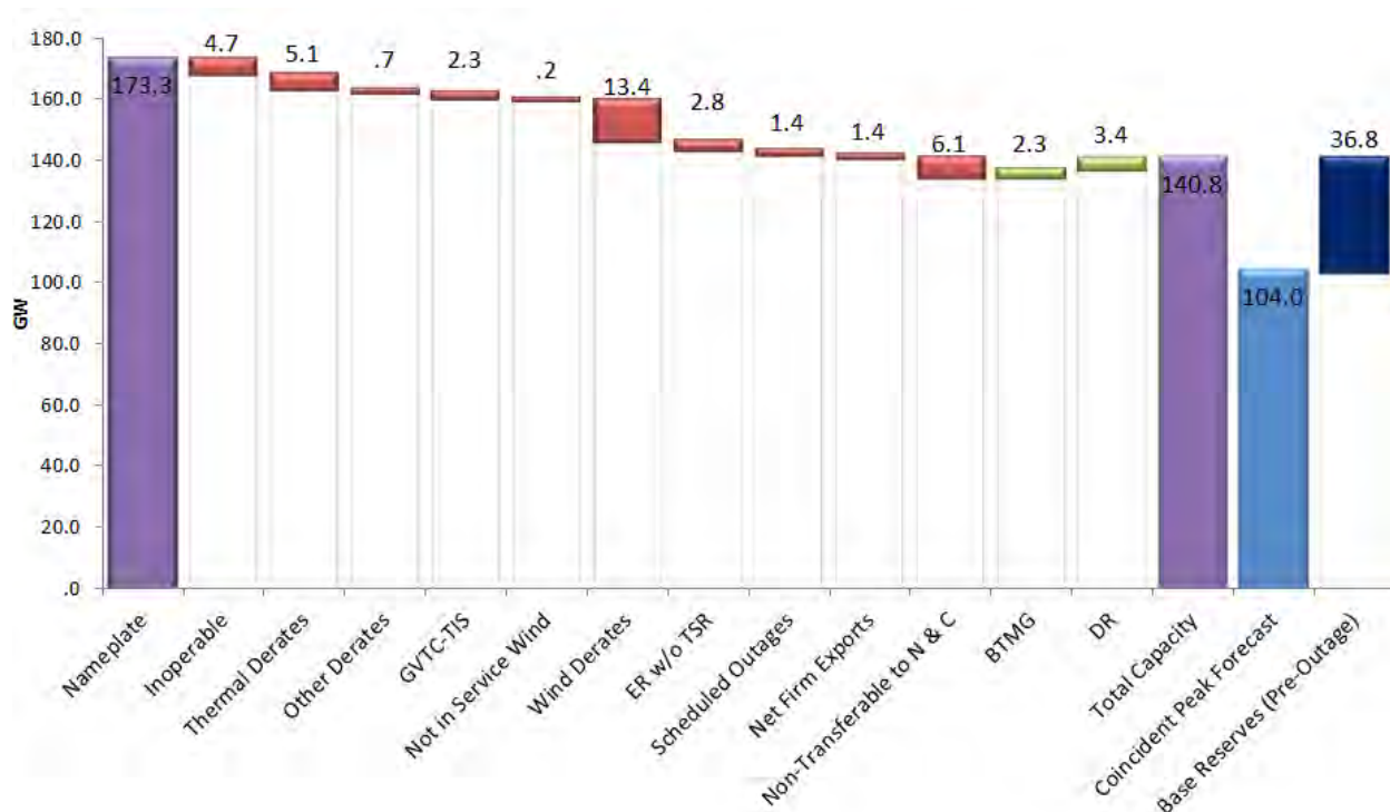
Figure 6.3-2: 2016-2017 Winter Rated Capacity projected Base scenario (GW)
