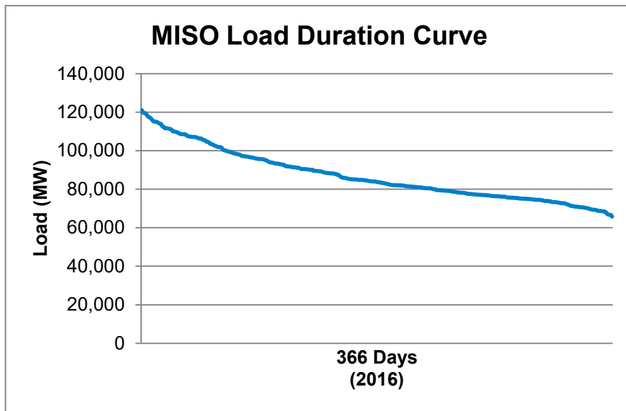
Figure 9.4-4: MISO Load Duration Curve – 2016 83
