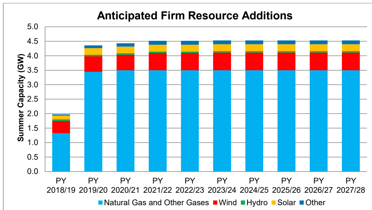
Figure 6.2-1: Anticipated Resource Additions and Uprates (Cumulative) of active projects with a signed Interconnection Agreement in the MISO Region
