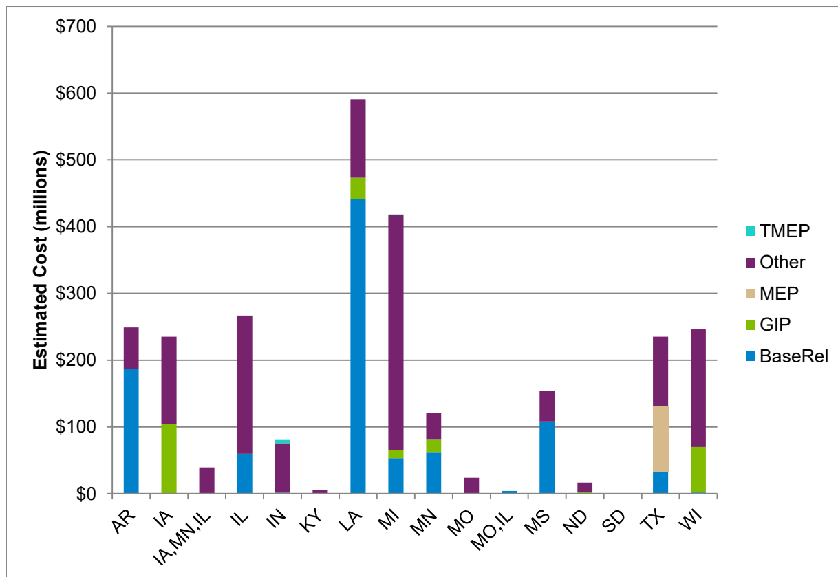
Figure 2.1-4: New MTEP17 Appendix A investment categorized by state
