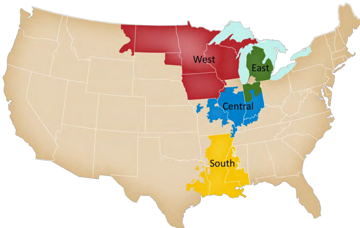
Figure 4.1-2: MISO planning subregions
