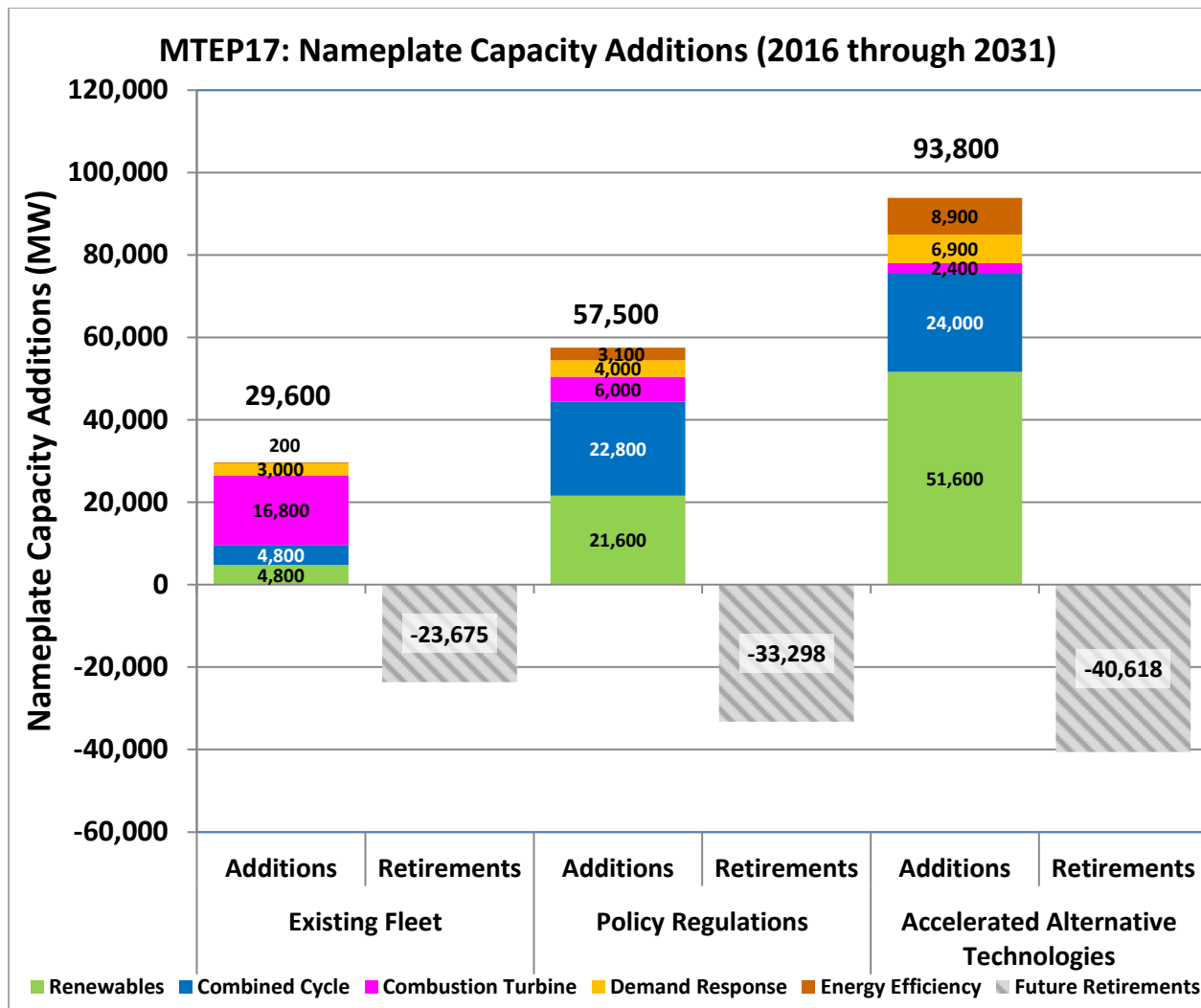
Figure 5.2-2: MISO nameplate capacity additions by future (2015-2030 EGEAS Model) 30
