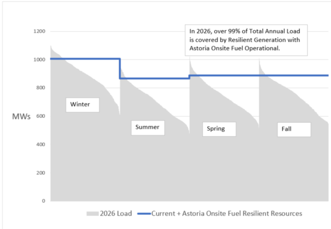
1 ADP Figure 3-10: 2026 Forecasted Load Relationship with Resilient 2 Generation (Current plus Astoria Onsite LNG Storage)
