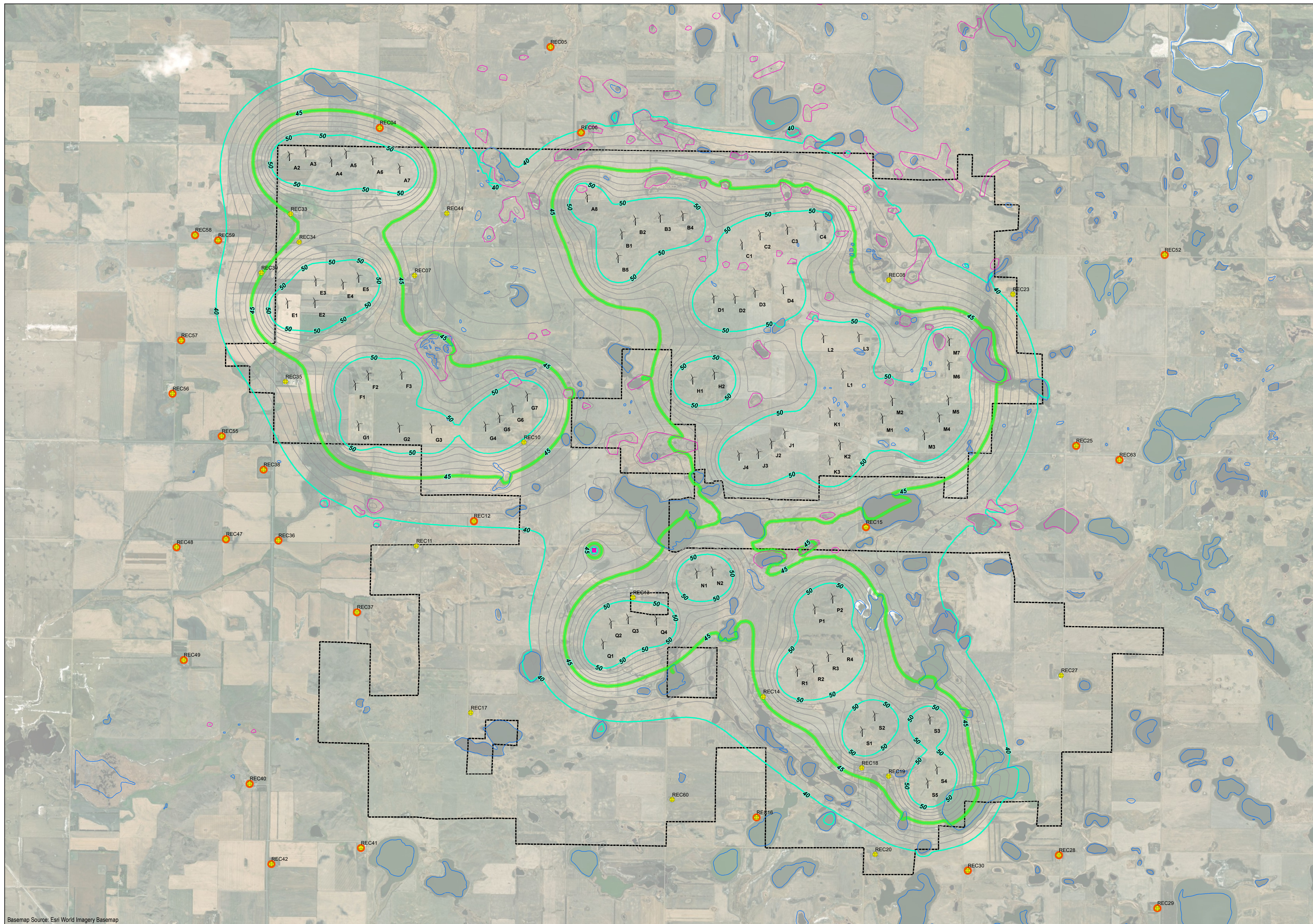
Figure 1 Predicted Sound Pressure Level (dBA) Vestas V120 Repower STE Blades Rugby Wind Repower Project
