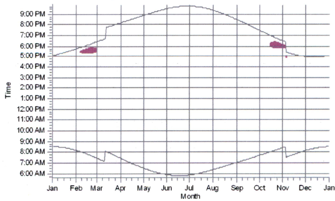
R015: Shadow Receptor: 1.0 × 1.0 Azimuth: 0.0° Slope: 90.0° (14)
