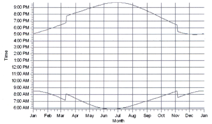
R148: Shadow Receptor: 1.0 × 1.0 Azimuth: 0.0° Slope: 90.0° (133)
