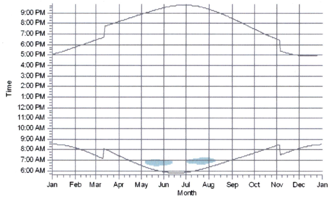
R092: Shadow Receptor: 1.0 × 1.0 Azimuth: 0.0° Slope: 90.0° (83)
