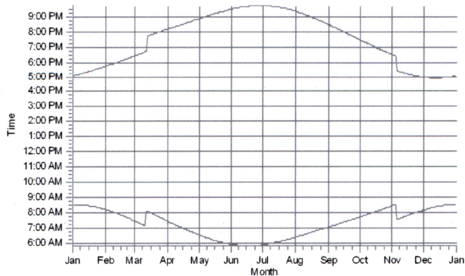
R130: Shadow Receptor: 1.0 × 1.0 Azimuth: 0.0° Slope: 90.0° (117)
