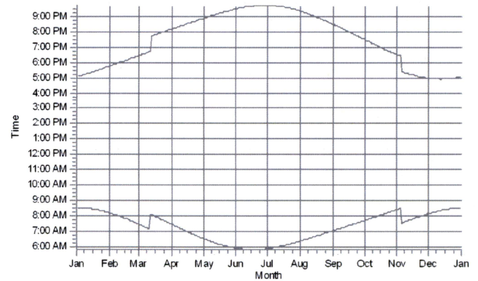
R093: Shadow Receptor: 1.0 × 1.0 Azimuth: 0.0° Slope: 90.0° (84)
