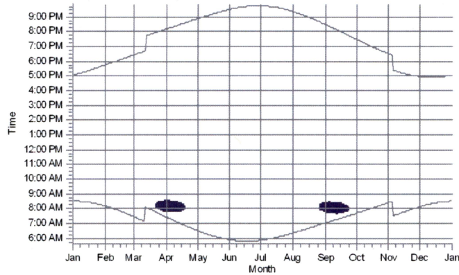
R098: Shadow Receptor: 1.0 × 1.0 Azimuth: 0.0° Slope: 90.0° (89)
