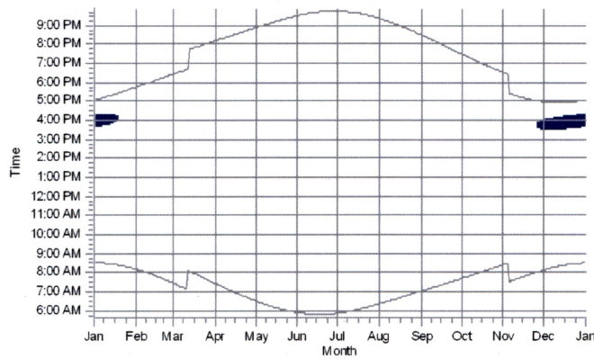
R107: Shadow Receptor: 1.0 × 1.0 Azimuth: 0.0° Slope: 90.0° (97)
