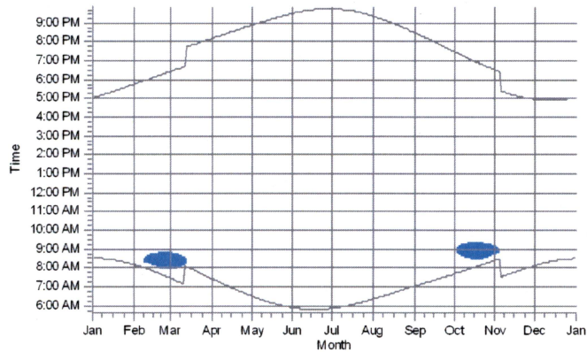
R157: Shadow Receptor: 1.0 × 1.0 Azimuth: 0.0° Slope: 90.0° (140)
