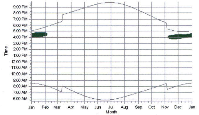
R035: Shadow Receptor: 1.0 × 1.0 Azimuth: 0.0° Slope: 90.0° (31)
