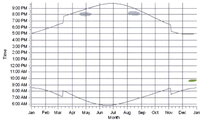
R143: Shadow Receptor: 1.0 × 1.0 Azimuth: 0.0° Slope: 90.0° (130)
