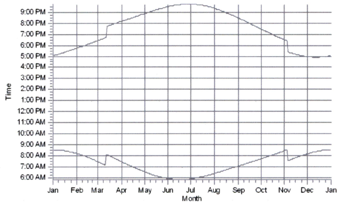
R126: Shadow Receptor: 1.0 × 1.0 Azimuth: 0.0° Slope: 90.0° (114)
