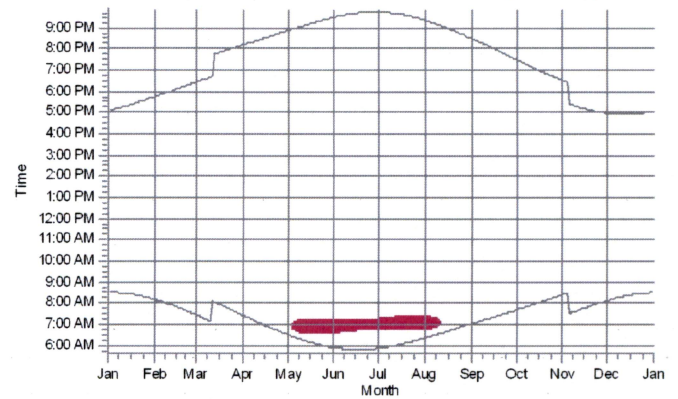
R095: Shadow Receptor: 1.0 × 1.0 Azimuth: 0.0° Slope: 90.0° (86)
