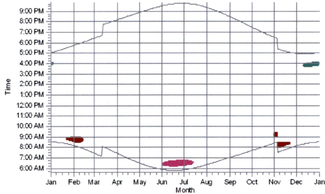
R117: Shadow Receptor: 1.0 × 1.0 Azimuth: 0.0° Slope: 90.0° (215)
