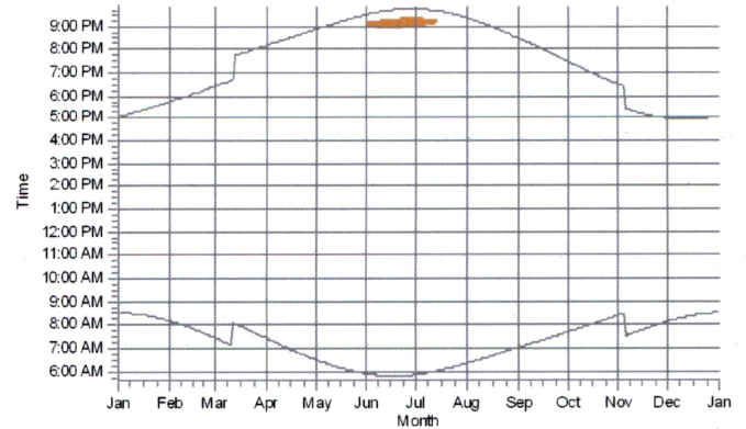
R122: Shadow Receptor: 1.0 × 1.0 Azimuth: 0.0° Slope: 90.0° (111)
