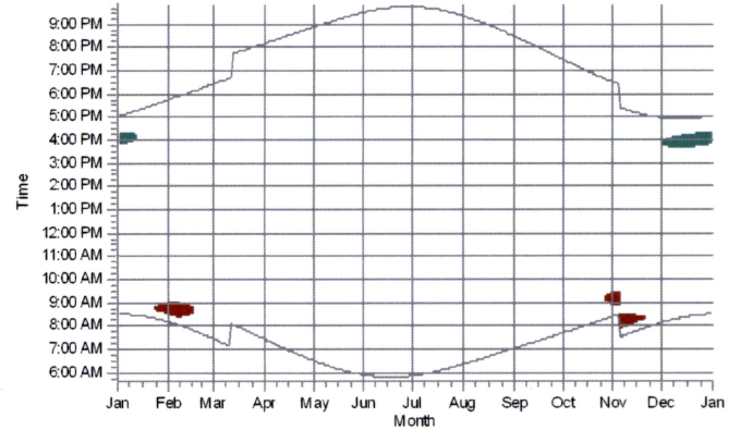
R118: Shadow Receptor: 1.0 × 1.0 Azimuth: 0.0° Slope: 90.0° (107)
