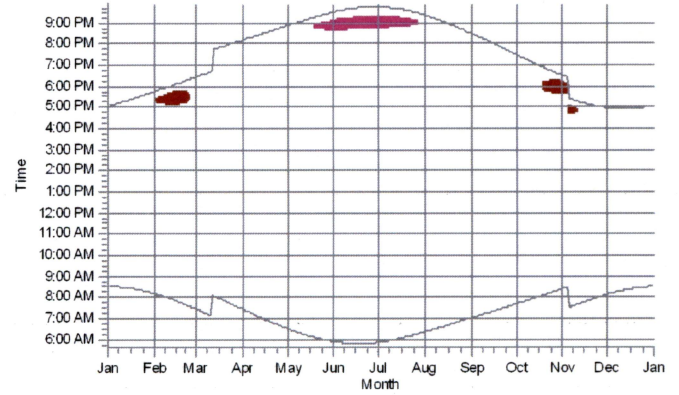
R120: Shadow Receptor: 1.0 × 1.0 Azimuth: 0.0° Slope: 90.0° (109)
