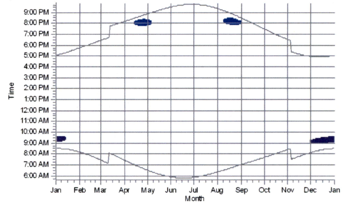
R100: Shadow Receptor: 1.0 × 1.0 Azimuth: 0.0° Slope: 90.0° (90)
