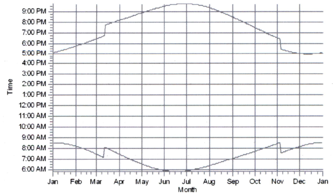
R131: Shadow Receptor: 1.0 × 1.0 Azimuth: 0.0° Slope: 90.0° (118)
