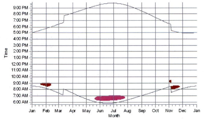
R116: Shadow Receptor: 1.0 × 1.0 Azimuth: 0.0° Slope: 90.0° (106)
