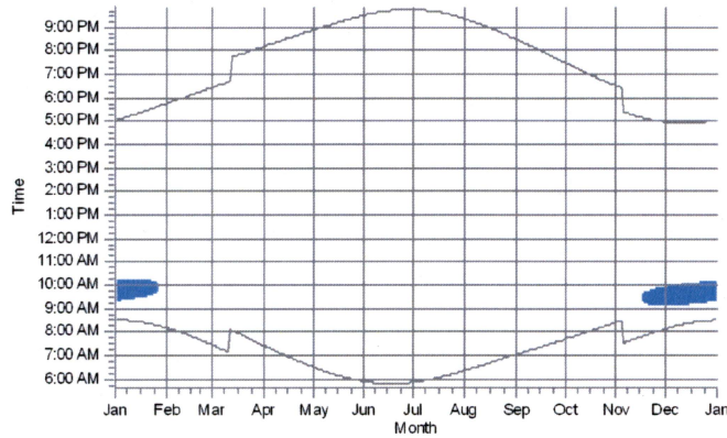
R105: Shadow Receptor: 1.0 × 1.0 Azimuth: 0.0° Slope: 90.0° (95)
