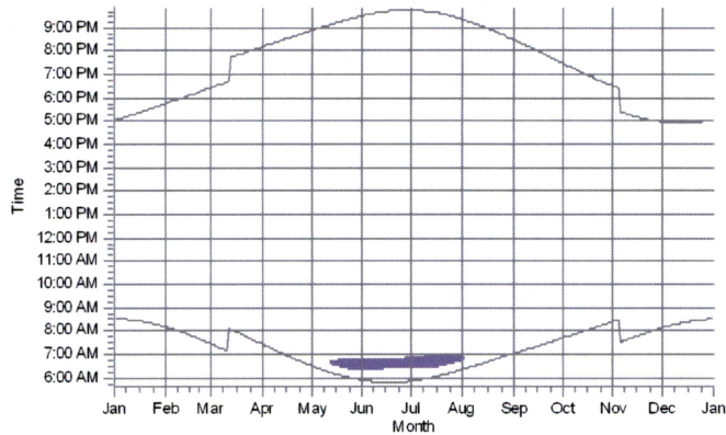
R123: Shadow Receptor: 1.0 × 1.0 Azimuth: 0.0° Slope: 90.0° (112)
