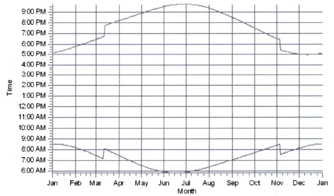
R110: Shadow Receptor: 1.0 × 1.0 Azimuth: 0.0° Slope: 90.0° (100)
