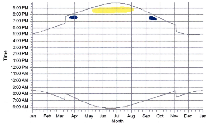
R101: Shadow Receptor: 1.0 × 1.0 Azimuth: 0.0° Slope: 90.0° (91)
