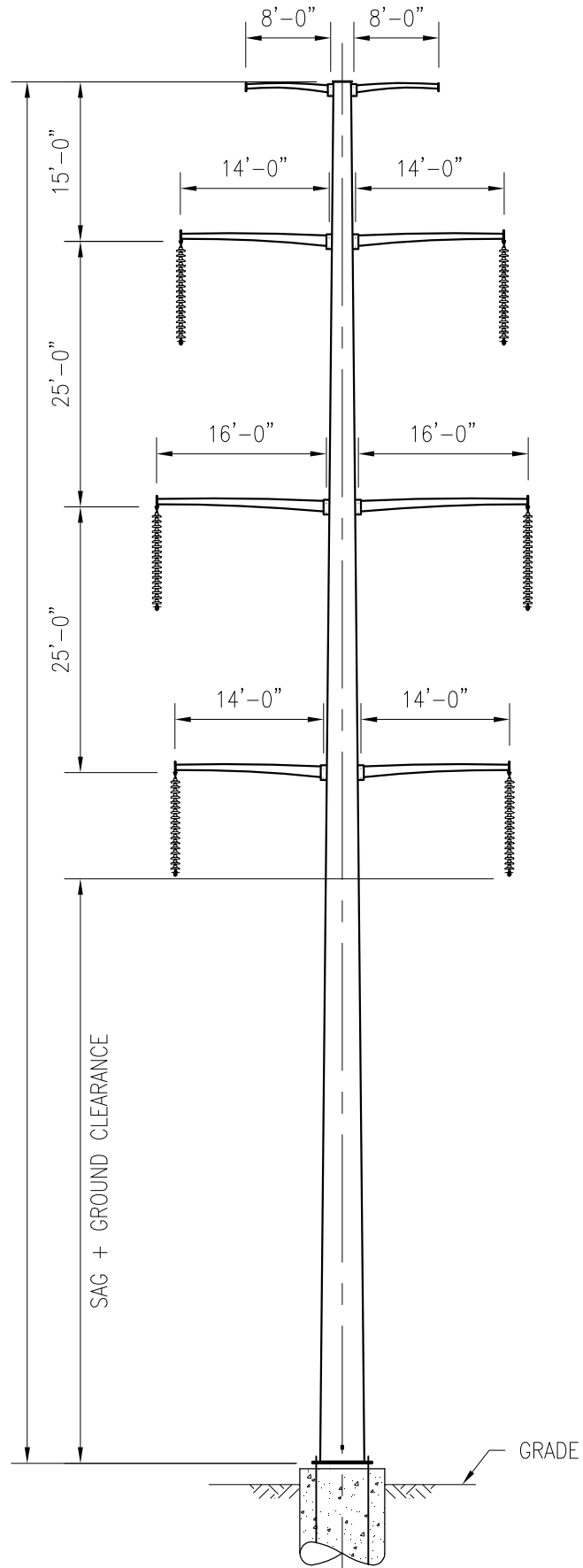
BASIC 345/345KV DOUBLE CIRCUIT STRUCTURE
