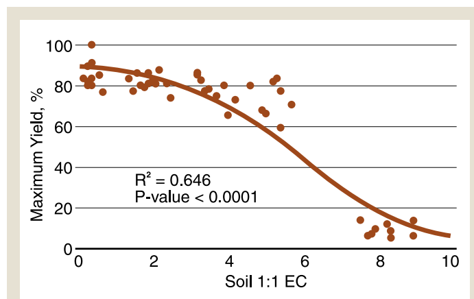
Figure 10. Relationship of spring wheat relative yield and soil 1:1 EC values. (Thapa et al., 2016)
