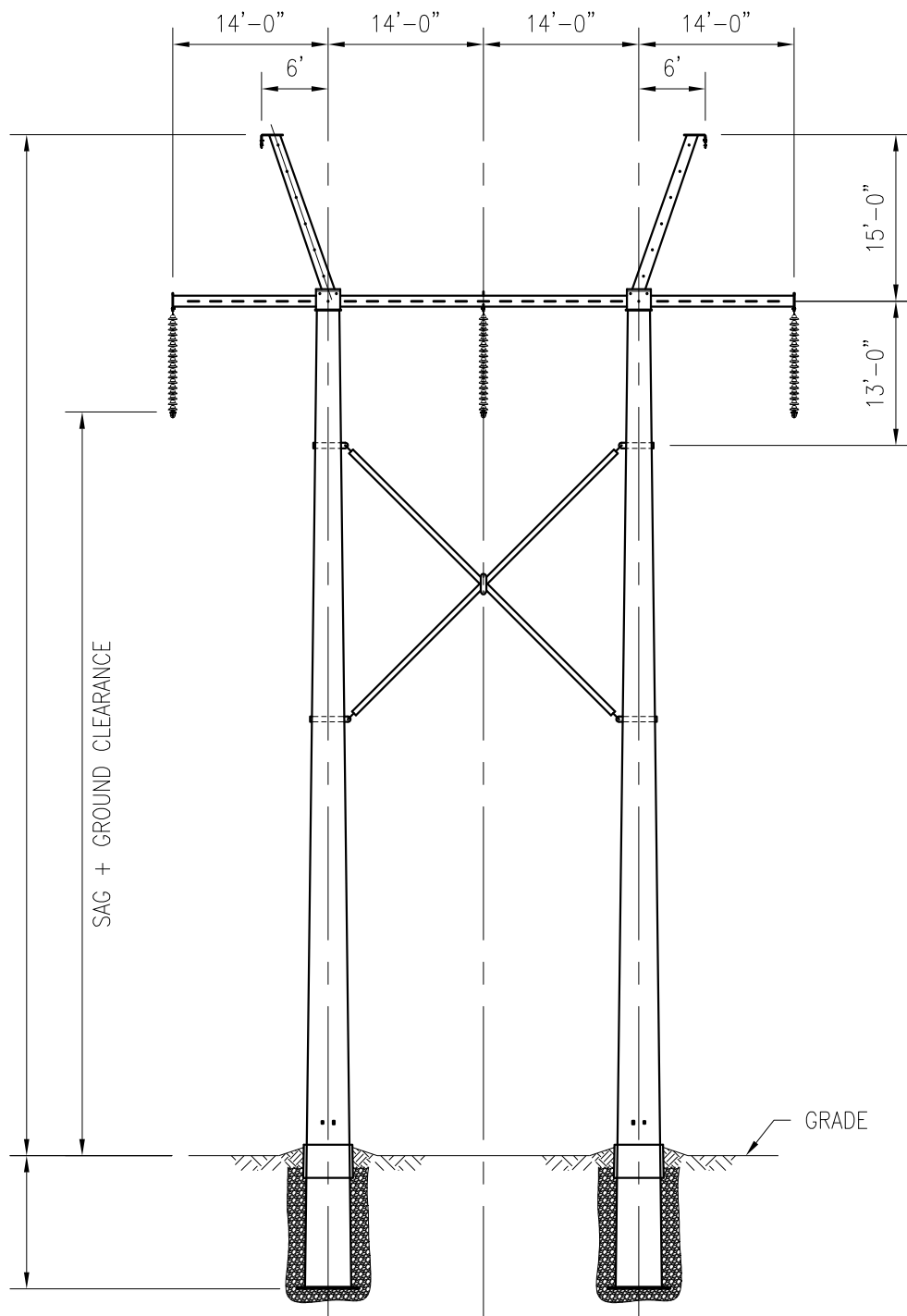
BASIC 345KV SINGLE CIRCUIT H-FRAME STRUCTURE
