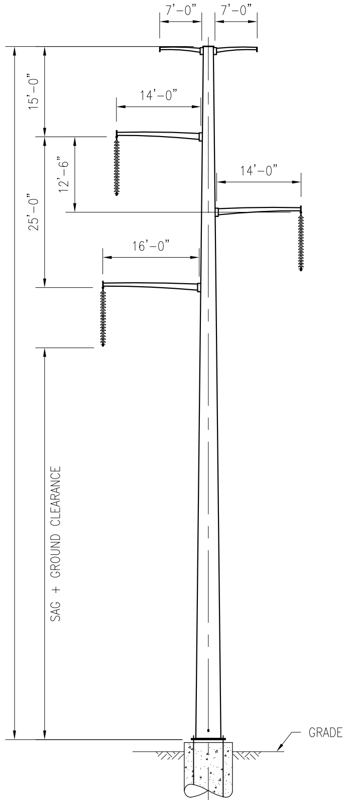
BASIC 345KV SINGLE CIRCUIT STRUCTURE
