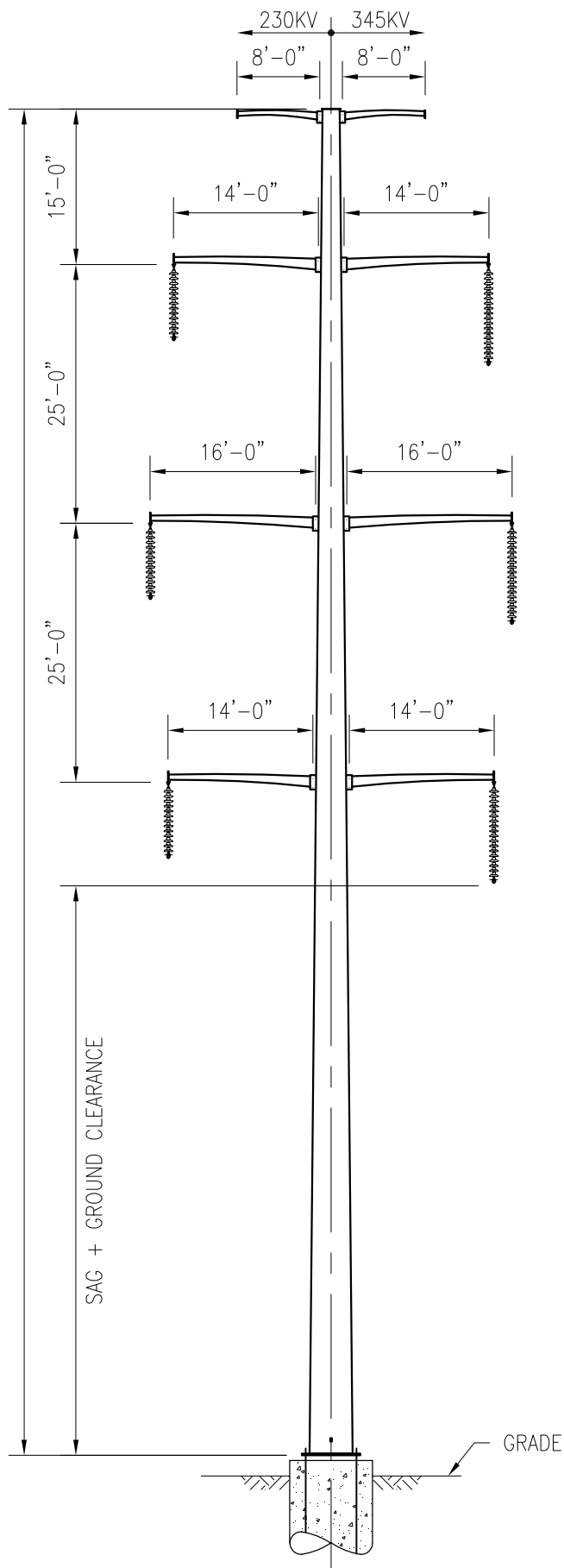
BASIC 345/230KV DOUBLE CIRCUIT TANGENT STRUCTURE
