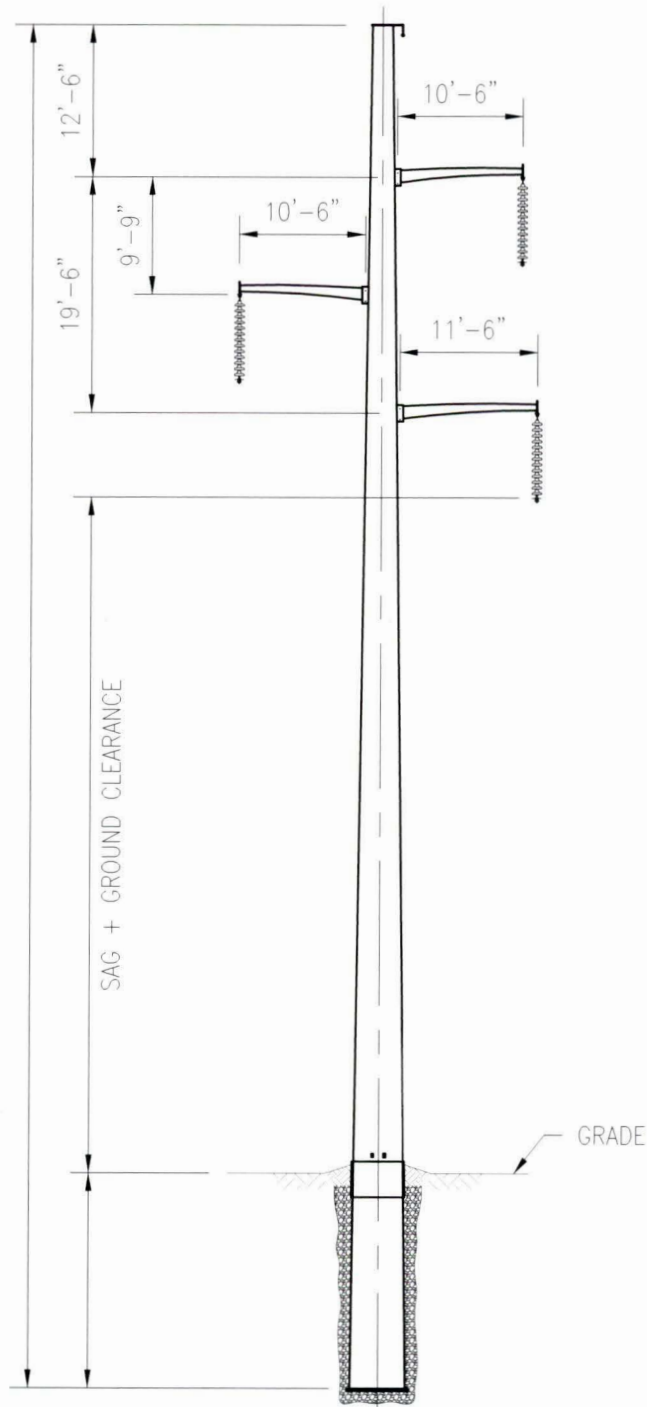
BASIC 230KV SINGLE CIRCUIT STRUCTURE
